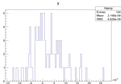
Figure 5: Orthogonality check of \alpha_x knob when introducing roll errors 800 urad.
