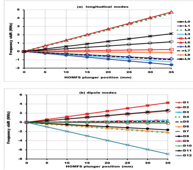
Figure 3: Frequency shift vs. HOMFS position (a) for monopole and (b) for dipole modes.
