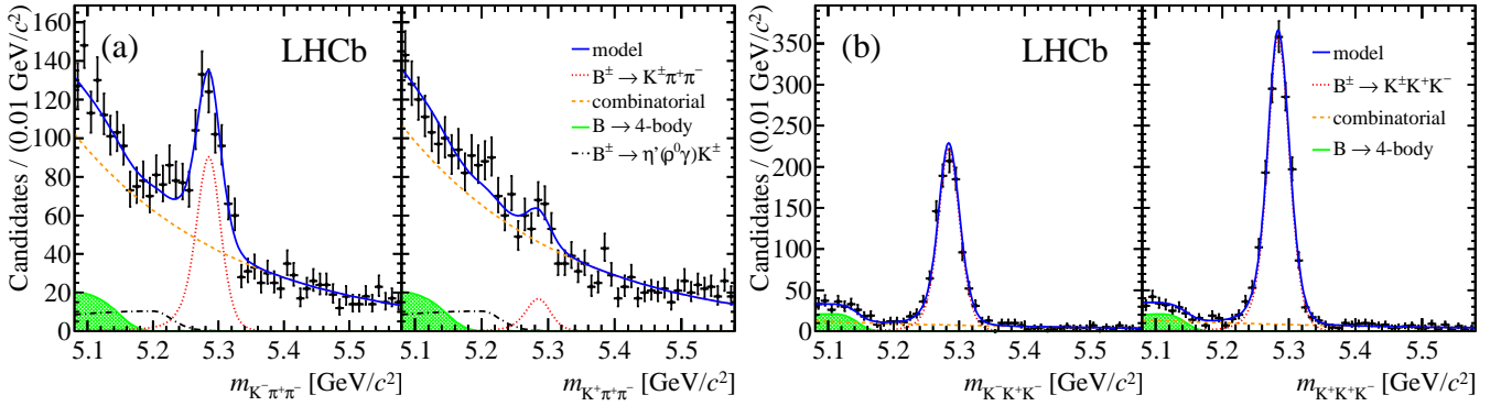
FIG. 3. Invariant mass spectra of (a) B^\pm \rightarrow K^\pm \pi^+ \pi^- decays in the region 0.08 < m_{\pi^+ \pi^-}^2 < 0.66 \text{ GeV}^2/c^4 and m_{K^\pm \pi^+ \pi^-}^2 < 15 \text{ GeV}^2/c^4 , and (b) B^\pm \rightarrow K^\pm K^+ K^- decays in the region 1.2 < m_{K^+ K^-}^2 < 2.0 \text{ GeV}^2/c^4 and m_{K^+ K^-}^2 < 15 \text{ GeV}^2/c^4 . The left panel in each figure shows the B^- modes and the right panel shows the B^+ modes. The results of the unbinned maximum likelihood fits are overlaid.
