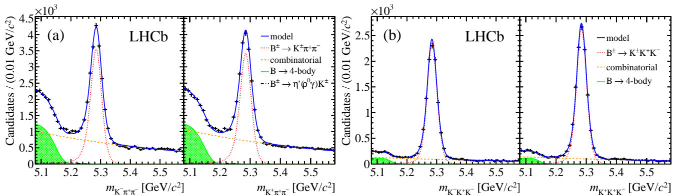
FIG. 1. Invariant mass spectra of (a) B^\pm \rightarrow K^\pm \pi^+ \pi^- decays and (b) B^\pm \rightarrow K^\pm K^+ K^- decays. The left panel in each figure shows the B^- modes and the right panel shows the B^+ modes. The results of the unbinned maximum likelihood fits are overlaid. The main components of the fit are also shown.
