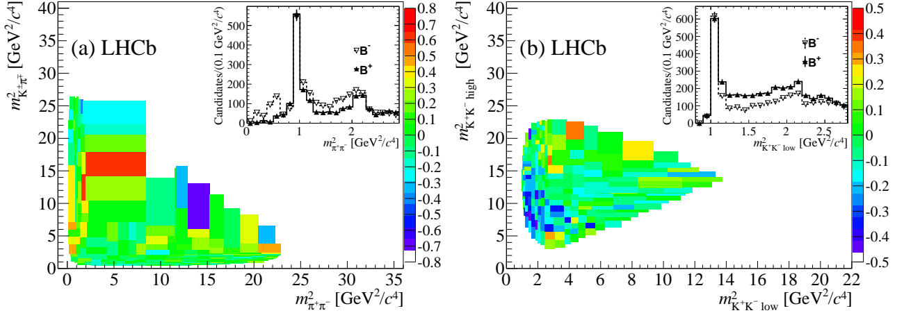
FIG. 2. Asymmetries of the number of signal events in bins of the Dalitz plot, A_{CP}^N , for (a) B^\pm \rightarrow K^\pm \pi^+ \pi^- and (b) B^\pm \rightarrow K^\pm K^+ K^- decays. The inset figures show the projections of the number of background-subtracted events in bins of (left) the m_{\pi^+ \pi^-}^2 variable for m_{K^\pm \pi^+ \pi^-}^2 < 15 \text{ GeV}^2/c^4 and (right) the m_{K^+ K^-}^2 variable for m_{K^+ K^-}^2 < 15 \text{ GeV}^2/c^4 . The distributions are not corrected for acceptance.
