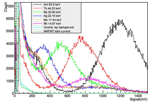
Fig. 5: The energy calibration for the YSO crystals using a variable X ray sources [8].
