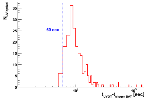
Fig. 1: The detected number of Swift's UV/optical events versus the response time of UVOT since 2005[3, 4].
