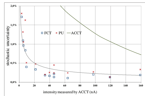
Figure 6: Stochastic uncertainty of measurement.
