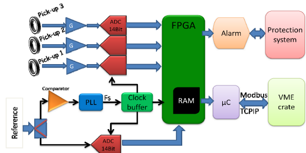
Figure 1: Electronic synoptic.
