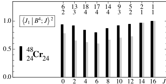
Fig. 9. The square of the projection of the yrast eigenstates in the (1f_{7/2})^8 system onto the subspace spanned by the B -pair states |B^4; J\rangle , for angular momentum J and isospin T = 0 . The shell-model interaction is defined in Eq. (39). Also shown are the numbers of (1f_{7/2})^8 states (top) and of B -pair states (bottom) with angular momentum J and isospin T = 0 . The grey bars represent the corresponding analysis in terms of the stretched configuration of Danos and Gillet 28,29 (see text).
