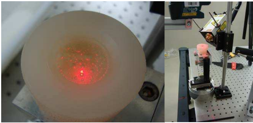
Figure 4: Left: Irradiation cell with H 2 bubbles produced by the water radiolysis, Right: In situ Raman spectroscopic device experiment under 4 He 2+ ions beam irradiation onto the ARRONAX facility vertical beam line
