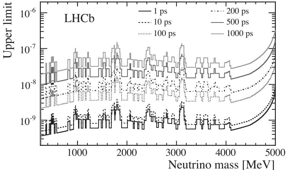
Figure 5: Upper limits on \mathcal{B}(B^- \rightarrow \pi^+ \mu^- \mu^-) at 95% C.L. as a function of m_N , in 5 MeV intervals, for specific values of \tau_N .
