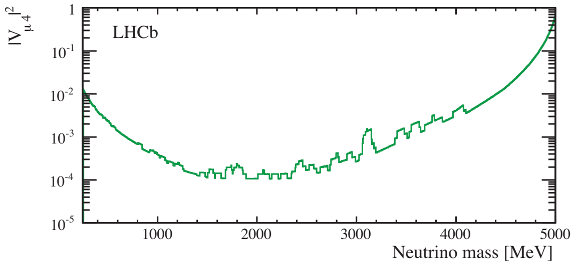
Figure 6: Upper limits at 95% C.L. on |V_{\mu 4}|^2 are shown as a function of m_N for \mathcal{L} events.
