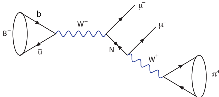
Figure 1: Feynman diagram for B^- \rightarrow \pi^+ \mu^- \mu^- decay via a Majorana neutrino labelled N .
