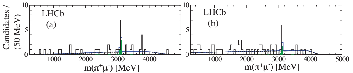
Figure 3: Invariant \pi^+\mu^- mass distribution for \pi^+\mu^-\mu^- candidates with masses restricted to \pm 2\sigma of B^- mass for the (a) \mathcal{S} and (b) \mathcal{L} selections. The shaded regions indicate the estimated peaking backgrounds. Backgrounds that peak under the signal in (a) and (b) are (green) shaded. The dotted lines show the combinatorial backgrounds only. The solid line the sum of both backgrounds. (In (a) there are two combinations per event.)
