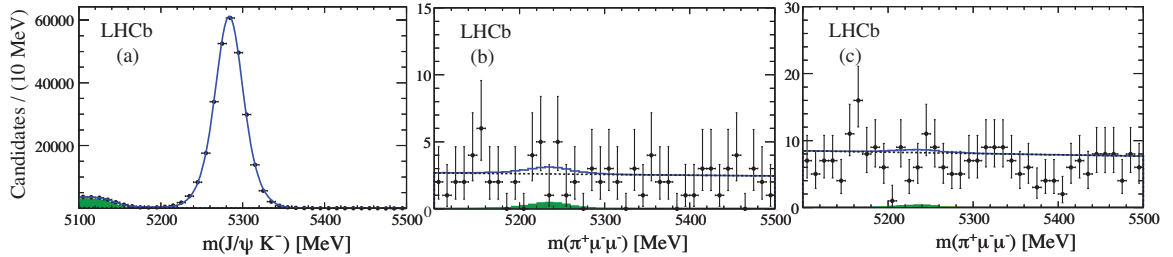
Figure 2: Invariant mass distributions with fits overlaid of candidate mass spectra for (a) J/\psi K^- , (b) \pi^+ \mu^- \mu^- ( \mathcal{S} ), and (c) \pi^+ \mu^- \mu^- ( \mathcal{L} ). Backgrounds are (green) shaded; they peak under the signal in (b) and (c). The dotted lines show the combinatorial backgrounds only. The solid line shows the sum of both backgrounds.
