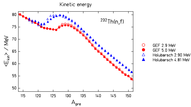
Figure 128: Mean total kinetic energy before evaporation as a function of the mass of the fragment for ^{232}\text{Th}(\text{n},\text{f}) [231].
