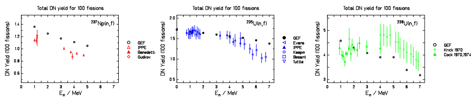
Figure 137: Delayed-neutron yields for ^{237}\text{Np}(n,f) , ^{235}\text{U}(n,f) and ^{238}\text{U}(n,f) , from [242] and references therein, in comparison with the GEF results.
