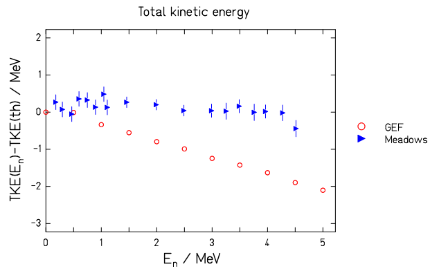
Figure 133: Difference between the total kinetic energy ( \text{TKE}(E_n) ) and the thermal value ( \text{TKE}(\text{th}) ) as a function of the neutron energy for ^{235}\text{U}(\text{n},\text{f}) [236].
