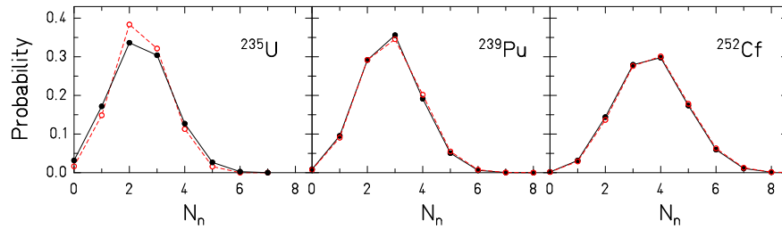
Figure 88: Measured distribution of prompt-neutron multiplicities in ^{235}\text{U}(n_{th},f) , ^{239}\text{Pu}(n_{th},f) and ^{252}\text{Cf}(sf) (data from refs. [173, 174]) (black full points) in comparison with the result of the GEF code (red open points).
