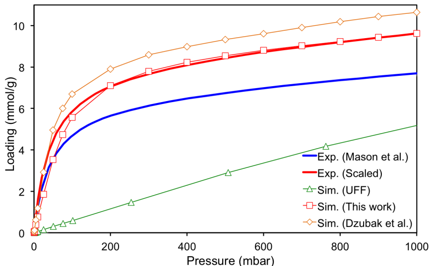
Figure 12: Isotherms of CO 2 adsorption in Mg-MOF-74. The experimental data was taken from ref 6 and was scaled assuming that 80 % of the sites within Mg-MOF-74 were available for adsorption of CO 2 as demonstrated by ref 15. The experiment was performed at 313 K, which was the temperature considered in each simulation.
