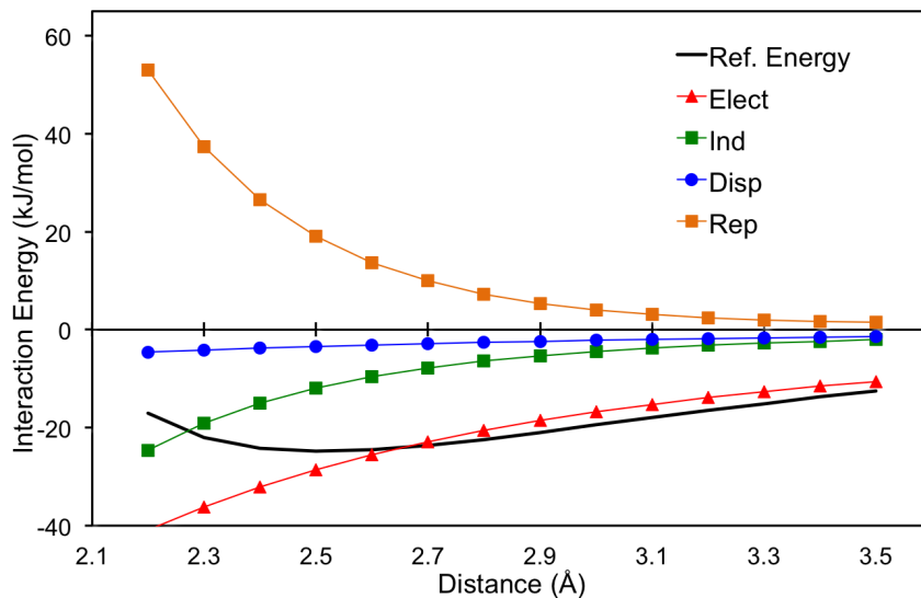
Figure 6: NEMO decomposition of the ROMP2 reference curve, including atomic dipole and quadrupole contributions, of the interaction of the 60-atom Fe-MOF-74 cluster with CO 2 .
