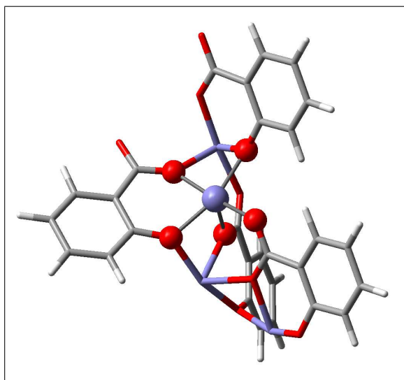
Figure 2: Sixty atom cluster used to model the Fe(II) ion and its ligand environment within Fe-MOF-74. Blue atoms represent iron, red are oxygen, grey are carbon, and white are hydrogen.
