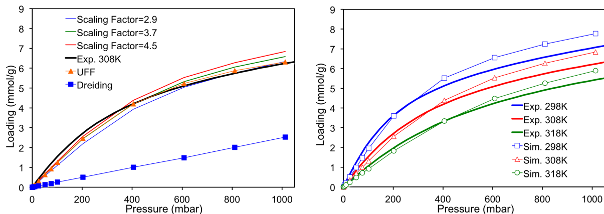
Figure 10: Experimental isotherm at 308 K is compared to the isotherm from the newly defined force field and the UFF and DREIDING force fields on the left. The picture on the left includes isotherms computed with different scaling factors on the dispersion term. The isotherms using the force field from this work are compared to experiment for multiple temperatures on the right.
