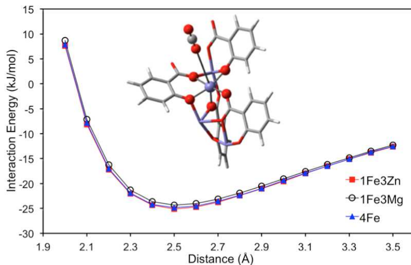
Figure 5: ROMP2 interaction energies computed for clusters in which the three non-central metal atoms were modeled by Mg(II) ions (black curve), Zn(II) ions (red curve), and Fe(II) ions (blue curve). A view of the CO 2 path as it approaches the MOF fragment is also provided.
