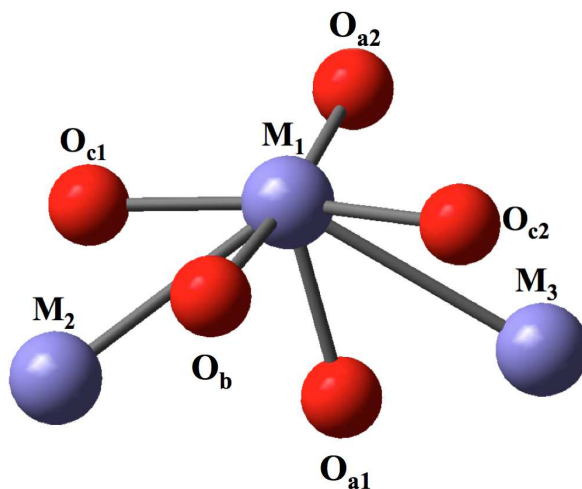
Figure 4: A single Fe(II) ion and its nearest neighbors within Fe-MOF-74. The O a , O b , and O c labels correspond to atom types described in Section S1. M 1 , M 2 , and M 3 are Fe(II) ions.
