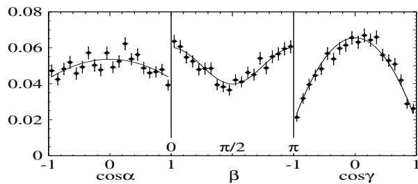
Figure 19.3.28. From (Balagura, 2008): Background-subtracted, efficiency-corrected and normalized one-dimensional projections of (\cos \alpha, \beta, \cos \gamma) described in the text. The solid curves show projections of the three-dimensional fit.
