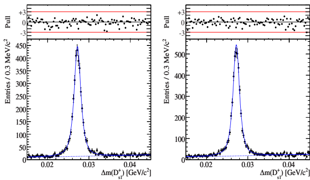
Figure 19.3.24. From (Lees, 2011d). \Delta m(D_{s1}(2536)^+) distribution for (left) the D^0 \rightarrow K^- \pi^+ \pi^+ \pi^- and (right) the D^0 \rightarrow K^- \pi^+ \pi^+ \pi^- decay modes. The solid line is the fit function as described in the text, the dotted line indicates the background contribution. The normalized fit residuals are shown on top.
