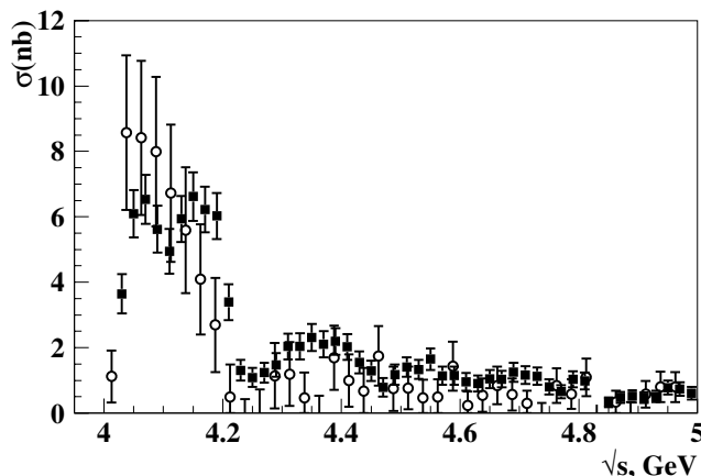
Figure 21.4.5. The exclusive cross sections for e^+e^- \rightarrow D^{*+}D^{*-} measured by Belle (Abe, 2007d; solid squares) and e^+e^- \rightarrow D^*\bar{D}^{*0} measured by BABAR (Aubert, 2009n; open circles).
