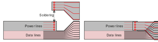
Figure 6.8: Power and data lines on the Inner Layers bus.
