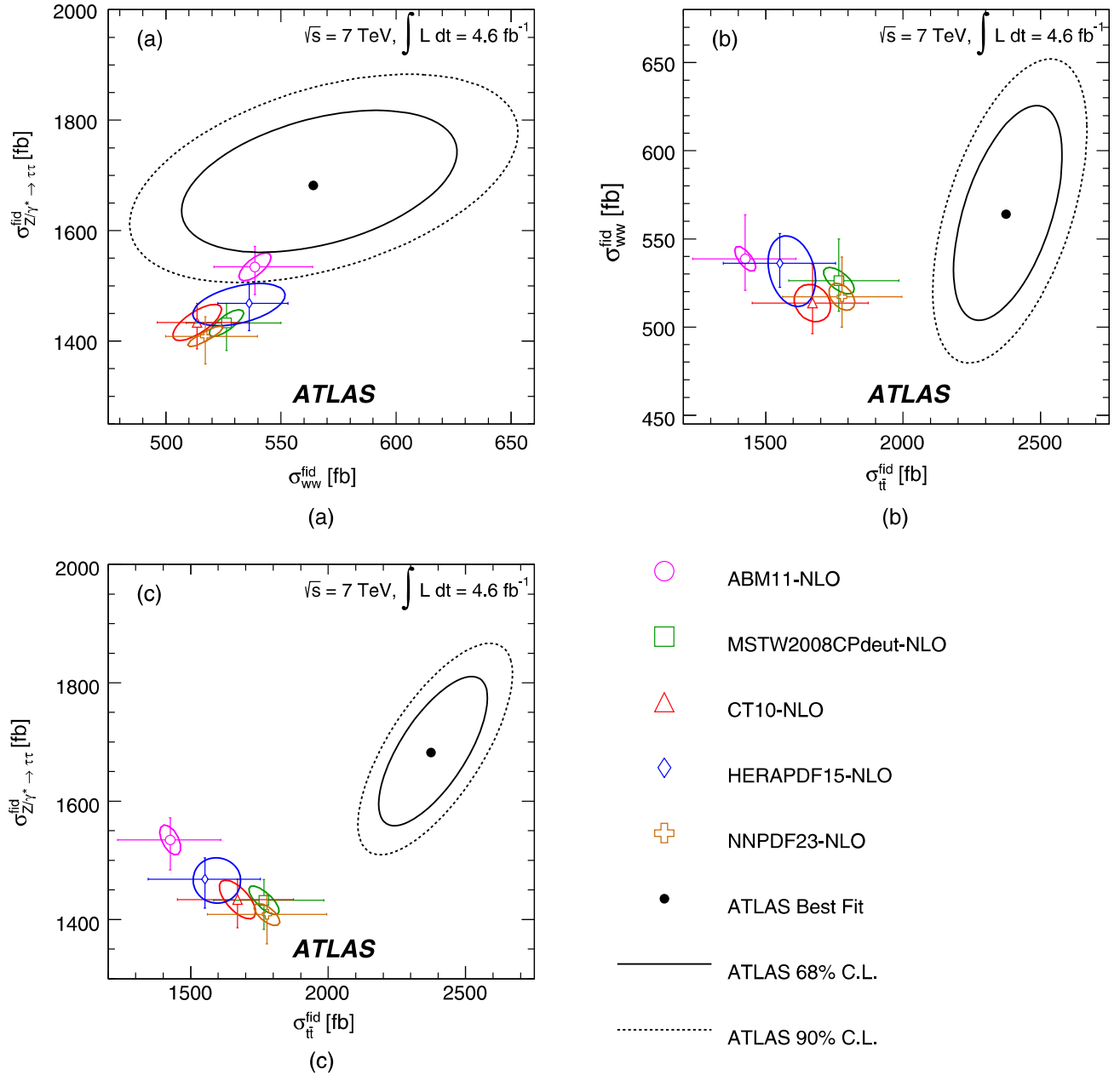
FIG. 6 (color online). Contours of the likelihood function as a function of two fiducial production cross-sections of interest: (a) \sigma_{Z/\gamma^* \to \tau\tau}^{\text{fid}} versus \sigma_{WW}^{\text{fid}} , (b) \sigma_{WW}^{\text{fid}} versus \sigma_{t\bar{t}}^{\text{fid}} , (c) \sigma_{Z/\gamma^* \to \tau\tau}^{\text{fid}} versus \sigma_{t\bar{t}}^{\text{fid}} . The contours obtained from the data (full circle) represent the 68 (full line) and 90% C.L. (dashed line) areas accounting for the full set of systematic uncertainties described in Table II. The fiducial cross-sections for WW and t\bar{t} exclude contributions from tau-lepton decays. The theoretical WW cross-section does not include contributions from gg \rightarrow H \rightarrow WW . The theoretical fiducial cross-section predictions are shown at NLO in QCD for different PDF sets (open symbols) with the ellipse contours corresponding to the 68% C.L. uncertainties on each PDF set. Also shown as horizontal and vertical error bars around each prediction are the uncertainties due to the choice of QCD factorization and renormalization scales (see text).
