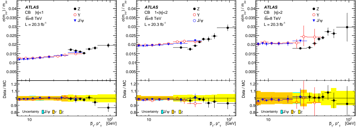
Fig. 14. Dimuon invariant mass resolution for CB muons measured from J/\psi , \Upsilon and Z events as a function of the average transverse momentum in three |\eta| ranges. Both muons are required to be in the same |\eta| range. The J/\psi and \Upsilon data are plotted as a function of \bar{p}_T = \frac{1}{2}(p_{T,1} + p_{T,2}) while for Z data are plotted as a function of p_T^* as defined in Eq. 16. The error bars represent statistical and systematic errors added in quadrature. The lower panel shows the ratio between data and the corrected MC, with bands representing the uncertainty on the MC corrections for the three calibration samples.
