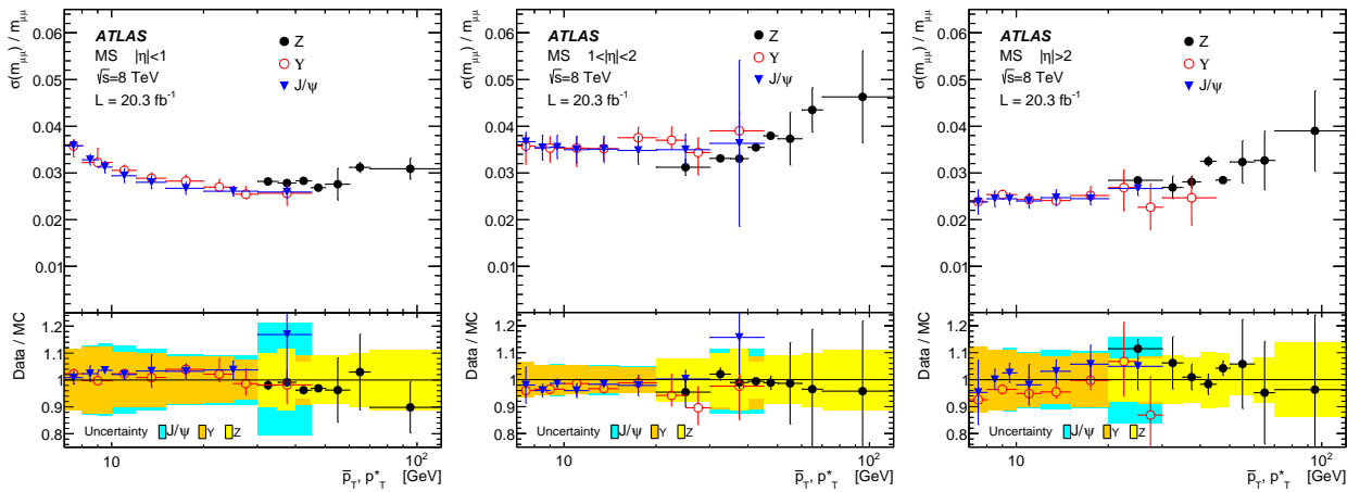
Fig. 16. Dimuon invariant mass resolution for muons reconstructed with the MS only, measured from J/\psi , \Upsilon and Z events as a function of the average transverse momentum in three |\eta| ranges. Other details as in Fig. 14.
