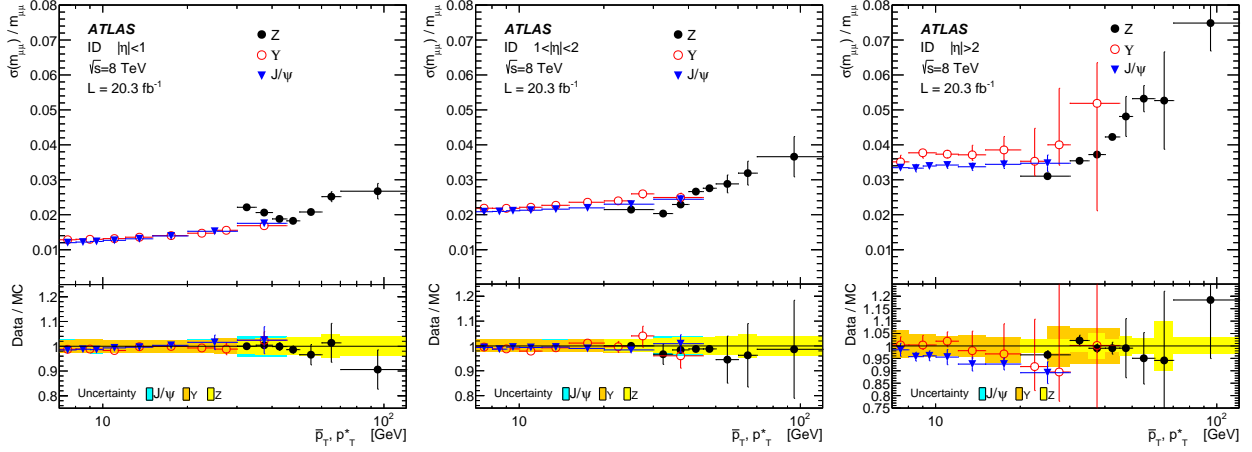
Fig. 15. Dimuon invariant mass resolution for muons reconstructed with the ID only, measured from J/\psi , \Upsilon and Z events as a function of the average transverse momentum in three |\eta| ranges. Other details as in Fig. 14.
