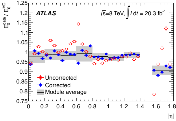
Fig. 15 Ratio of the average PS energies, E_0^{\text{data}}/E_0^{\text{MC}} , for electrons in data and simulation as a function of |\eta| , before and after corrections for b_{1/2} and material upstream of the PS. The full lines with shaded bands represent the PS energy scale as a function of |\eta| , \alpha_{\text{PS}}(\eta) , and its uncertainty.
