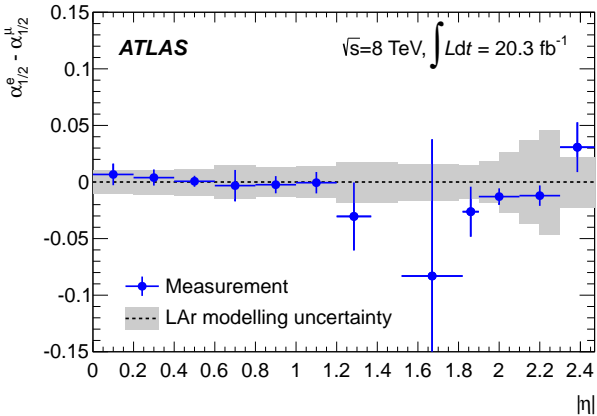
Fig. 17 Difference between the electron- and muon-based L1/L2 calibration results, denoted \alpha_{1/2}^e and \alpha_{1/2}^{\mu} respectively, as a function of |\eta| . The uncertainty band reflects the systematic uncertainties affecting the muon result; the error bars represent the uncertainty on the electron result.
