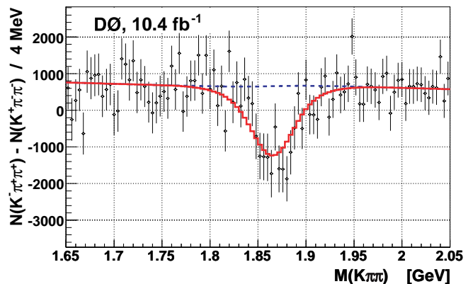
FIG. 2: Invariant mass distribution M(K\pi\pi) for the difference N(D^+) - N(D^-) (data markers). Also shown are the result of the fit to the data (solid line) and the overall background contribution (dashed line).
