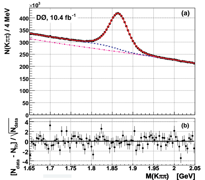
FIG. 1: (a) Invariant mass distribution M(K\pi\pi) after all selections have been applied (data markers). Also shown is the result of the fit to the data, as described in the text (solid line). To illustrate the contributions of the three separate components, the total background (dashed line) and polynomial function (dot-dashed line) are shown separately. (b) Fit residuals [N_{\text{data}} - N_{\text{fit}}] / \sqrt{N_{\text{data}}} , demonstrating the agreement between the data and the fit model.
