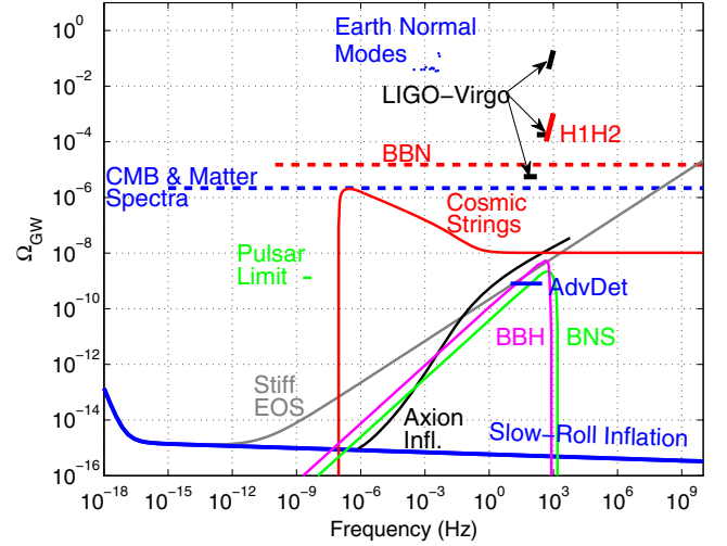
FIG. 10 (color online). Upper limits from the current H1-H2 analysis, previous SGWB analyses and the projected advanced LIGO limit, along with various SGWB models. The BBN limit is an integral limit on \Omega_{\text{gw}} i.e., \int \Omega_{\text{gw}}(f) d(\ln f) in the 10^{-10} – 10^{10} Hz band derived from the big bang nucleosynthesis and observations of the abundance of light nuclei [28,49]. The measurements of CMB and matter power spectra provide a similar integral bound in the frequency range of 10^{-15} – 10^{10} Hz [50]. The pulsar limit is a bound on the \Omega_{\text{gw}}(f) at f = 2.8 nHz and is based on the fluctuations in the pulse arrival times from millisecond pulsars [51]. In the above figure, the slow-roll inflationary model [52] assumes a tensor-to-scalar ratio of r = 0.2 , the best fit value from the BICEP2 analysis [13]. In the axion based inflationary model, for certain ranges of parameters the backreaction during the final stages of inflation is expected to produce strong GWs at high frequencies [53]. The stiff equation of state (EOS) limit corresponds to scenarios in the early Universe (prior to BBN) in which GWs are produced by an unknown “stiff” energy [54]. For the above figure we used the equation of state parameter w = 0.6 in the stiff EOS model. The cosmic string model corresponds to GWs produced by cosmic strings in the early Universe [55]. The Earth’s normal mode limits are based on the observed fluctuations in the amplitudes of Earth’s normal modes using an array of seismometers [56]. The astrophysical SGWBs (BBH and BNS) are due to the superposition of coalescence GW signals from a large number of binary black holes (BBH) and binary neutron stars (BNS) [57].
