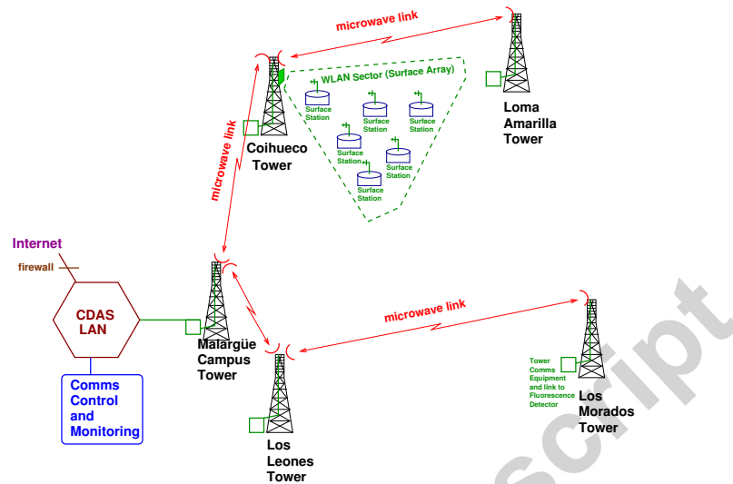
Figure 11: Conceptual schematic of the overall radio telecommunications system for the Pierre Auger Observatory.
