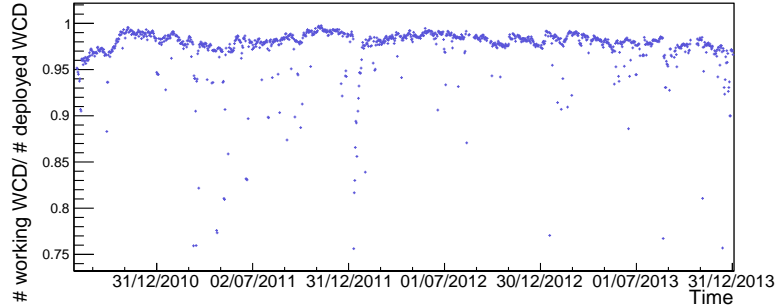
Figure 42: Number of active SD stations normalized to the nominal number of SD stations in the array, as a function of time. (Note: WCD = water Cherenkov detector.)
