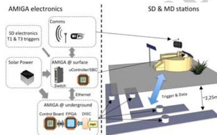
Figure 53: AMIGA station: SD+MD paired detectors. During the MD prototype phase the 30\text{ m}^2 buried scintillators are segmented into 4 modules, 2 \times 10\text{ m}^2 + 2 \times 5\text{ m}^2 . To avoid shadowing effects by the water Cherenkov detector, there are 5 m of sideways clearance. The buried front end electronics is serviceable by means of an access pipe which is filled with local soil bags. Data are sent by a dedicated WiFi antenna.
