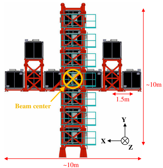
FIG. 3 (color online). Overview of the INGRID viewed from beam upstream. Two separate modules are placed at off-axis positions off the main cross to monitor the asymmetry of the beam.
