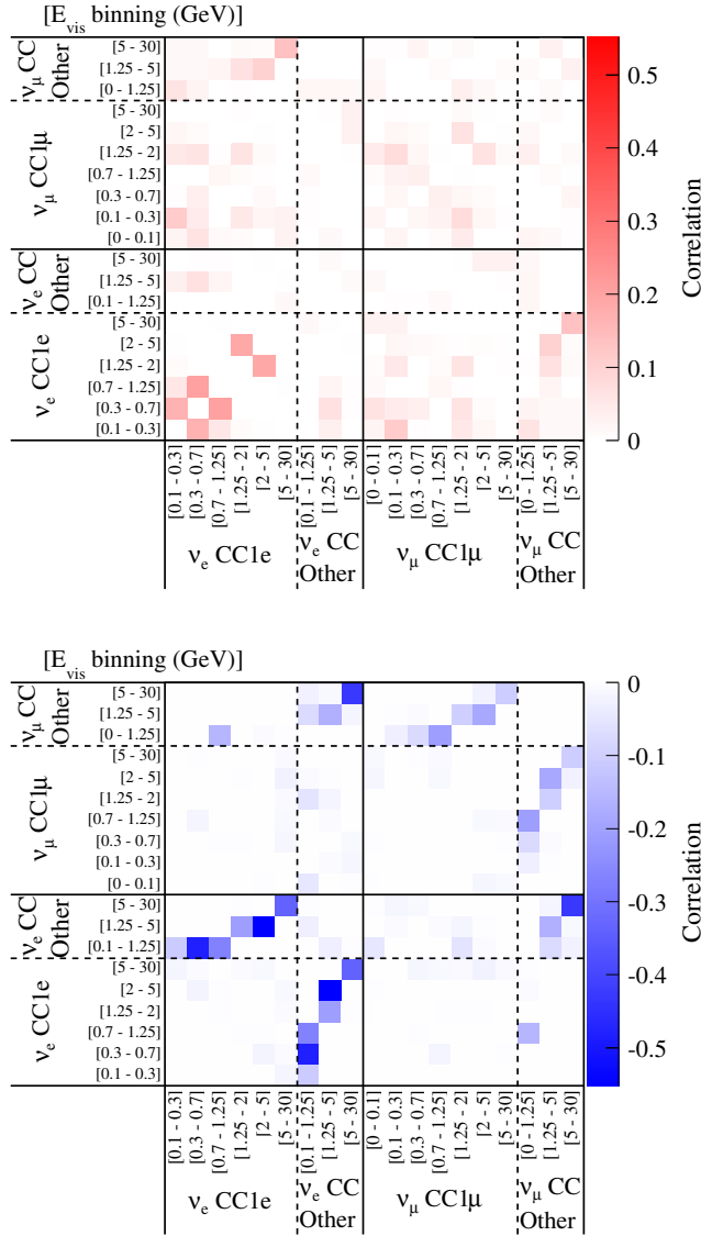
FIG. 24 (color online). The correlations between the estimated efficiencies for the final state topologies CC1e and CCe other for the \nu_e CC event selection and CC1 \mu and CC \mu other for the \nu_\mu CC event selection. The upper figure shows the combinations with positive correlation, and the lower with negative correlation. The diagonal correlations (correlation = 1) are not shown.
