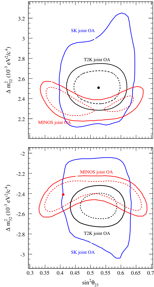
FIG. 36 (color online). The 68% (dashed) and 90% (solid) C.L. regions for normal (top) and inverted (bottom) mass hierarchy combined with the results from reactor experiments in the (\sin^2 \theta_{23}, \Delta m_{32}^2) space compared to the results from the Super-Kamiokande [131] and MINOS [132] experiments.
