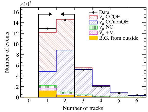
FIG. 5 (color online). The number of reconstructed tracks from the vertex in the proton module. The colored histograms are the MC predictions divided by the neutrino type and interaction type. The neutrino interaction events in the proton module are absolutely normalized to POT, and the background events from outside are normalized to beam induced muon backgrounds.
