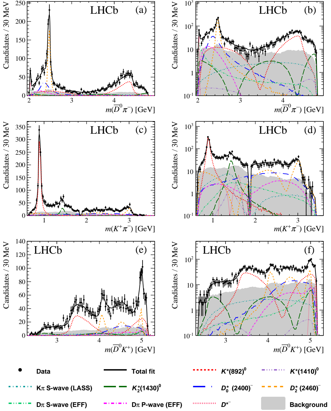
Figure 6: Projections of the data and amplitude fit results onto (a) m(\bar{D}^0\pi^-) , (c) m(K^+\pi^-) and (e) m(\bar{D}^0K^+) , with the same projections shown in (b), (d) and (f) with a logarithmic y -axis scale. Components are described in the legend.
