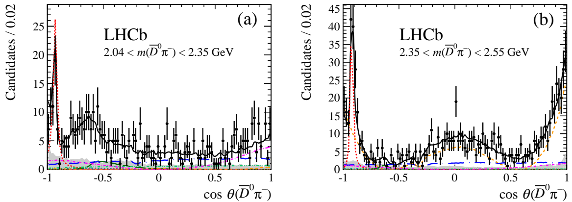
Figure 8: Projections of the data and amplitude fit results onto \cos\theta(\bar{D}^0\pi^-) in the mass ranges (a) 2.04 < m(\bar{D}^0\pi^-) < 2.35 GeV and (b) 2.35 < m(\bar{D}^0\pi^-) < 2.55 GeV. Components are as shown in Fig. 6.
