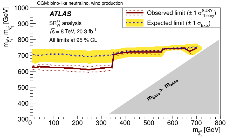
Figure 9: Exclusion limits in the wino-bino mass plane, using the SR_{W-H}^{\gamma\gamma} analysis for m_{\tilde{\chi}_1^0} \geq 350 \text{ GeV} and the SR_{W-L}^{\gamma\gamma} analysis for m_{\tilde{\chi}_1^0} < 350 \text{ GeV} . The vertical axis represents wino mass while the horizontal axis represents bino mass. The observed limits are exhibited for the nominal SUSY model cross-section expectation, as well as for a SUSY cross section increased and decreased by 1 standard-deviation of the cross-section systematic uncertainty. Also shown is the expected limit, along with its \pm 1 standard-deviation range. The discontinuity at m_{\tilde{\chi}_1^0} = 350 \text{ GeV} is due to the switch between the use of the SR_{W-L}^{\gamma\gamma} and SR_{W-H}^{\gamma\gamma} analyses, the former of which exhibits a small excess of observed events relative to the expected SM background.
