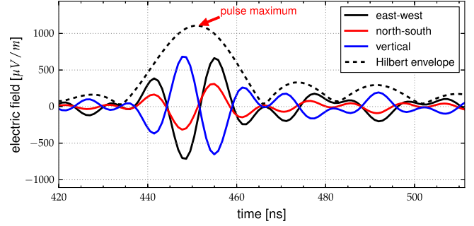
FIG. 1. Reconstructed electric-field trace of one of the measured cosmic-ray radio events. An upsampling by a factor of 5 was applied. The shown Hilbert envelope (dashed line) is the square root of the quadratic sum of the Hilbert envelopes of the three polarization components.
