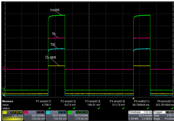
Figure 3: Typical scope traces of diode detectors and electron probe.
