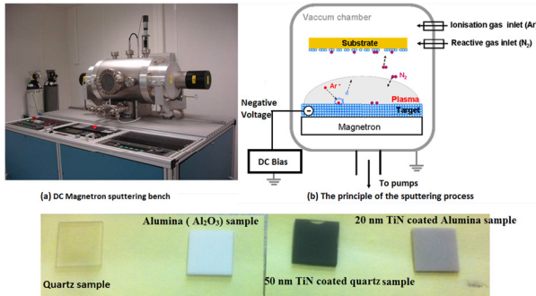
Figure 1: View of the DC Magnetron sputtering bench.
