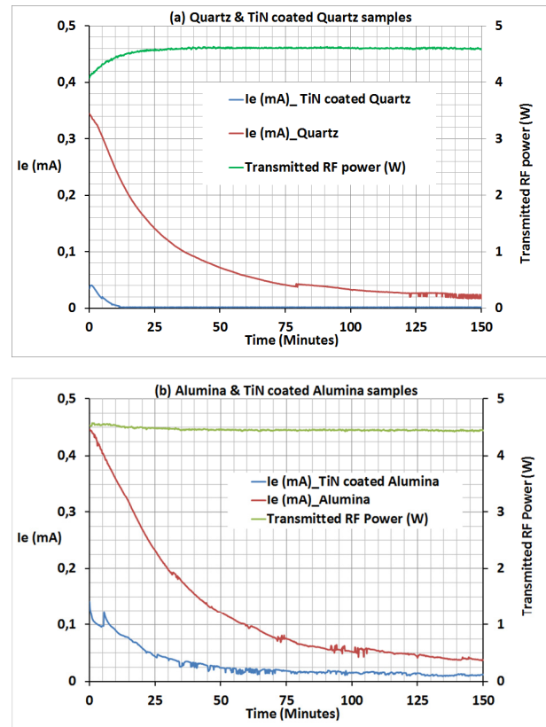
Figure 5: Multipacting current vs. time for a constant transmitted RF power (a) Quartz & TiN (50 nm) coated Quartz; (b) Alumina & TiN (20 nm) coated Alumina.
