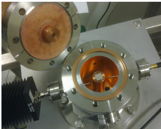
Figure 4: View of the RF coaxial resonator with a dielectric sample holder.
