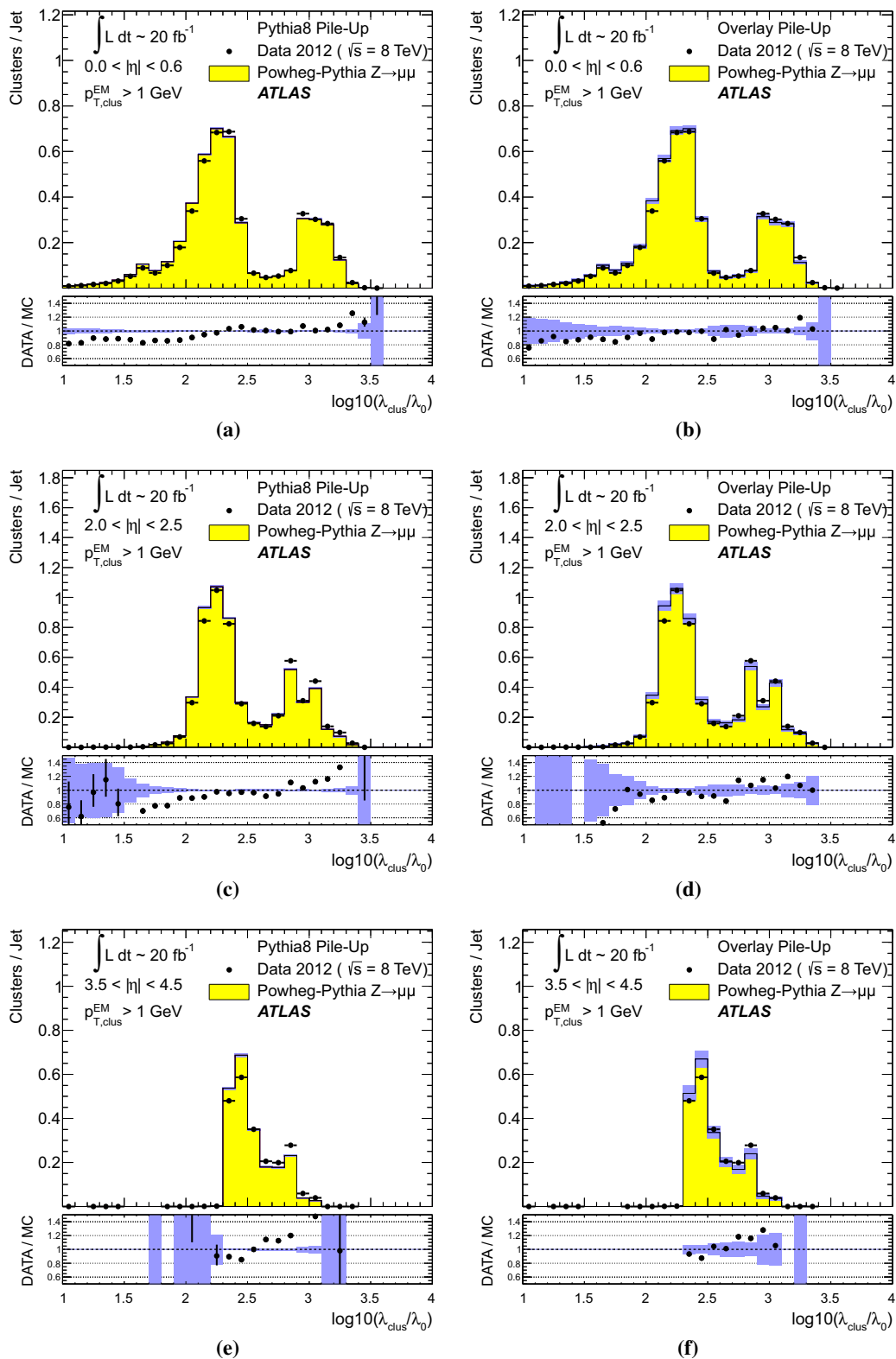
Fig. 35 The distribution of the depth location, measured in terms of \log_{10}(\lambda_{\text{clus}}/\lambda_0) with \lambda_0 = 1 mm, of topo-clusters with p_{T,\text{clus}}^{\text{EM}} > 1 GeV in jets reconstructed with the anti- k_r algorithm with R = 0.4 and with 30 \text{ GeV} < p_{T,\text{jet}}^{\text{LCW+JES}} < 40 \text{ GeV} in Z \rightarrow \mu\mu events in 2012 data and MC simulations with (a, c, e) fully simulated pile-up and with (b, d, f) overlaid pile-up from data. Distributions are shown for jets in the (a, b)
