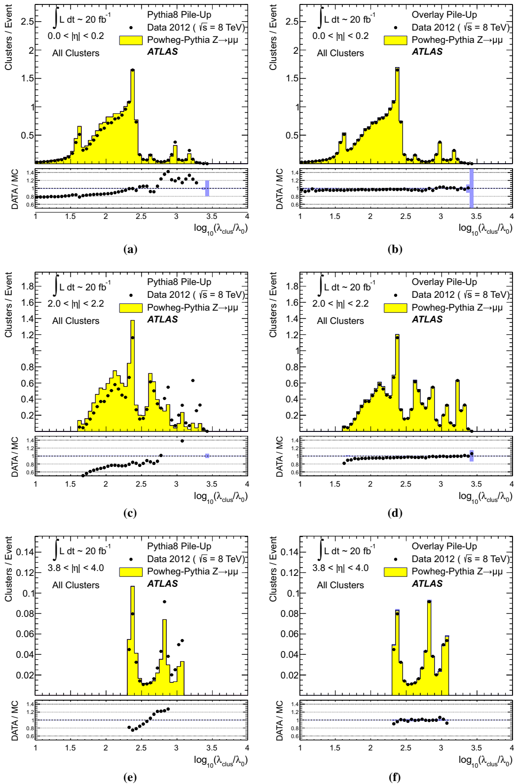
Fig. 28 The distribution of the topo-cluster depth location, measured in terms of \log_{10}(\lambda_{clus}/\lambda_0) , for clusters in various bins of \eta_{clus} for an inclusive Z \rightarrow \mu\mu event sample recorded in 2012. Data is compared to distributions from MC simulations including fully simulated pile-up for all topo-clusters within a |\eta_{clus}| < 0.2 , c 2.0 < |\eta_{clus}| < 2.2 , and
