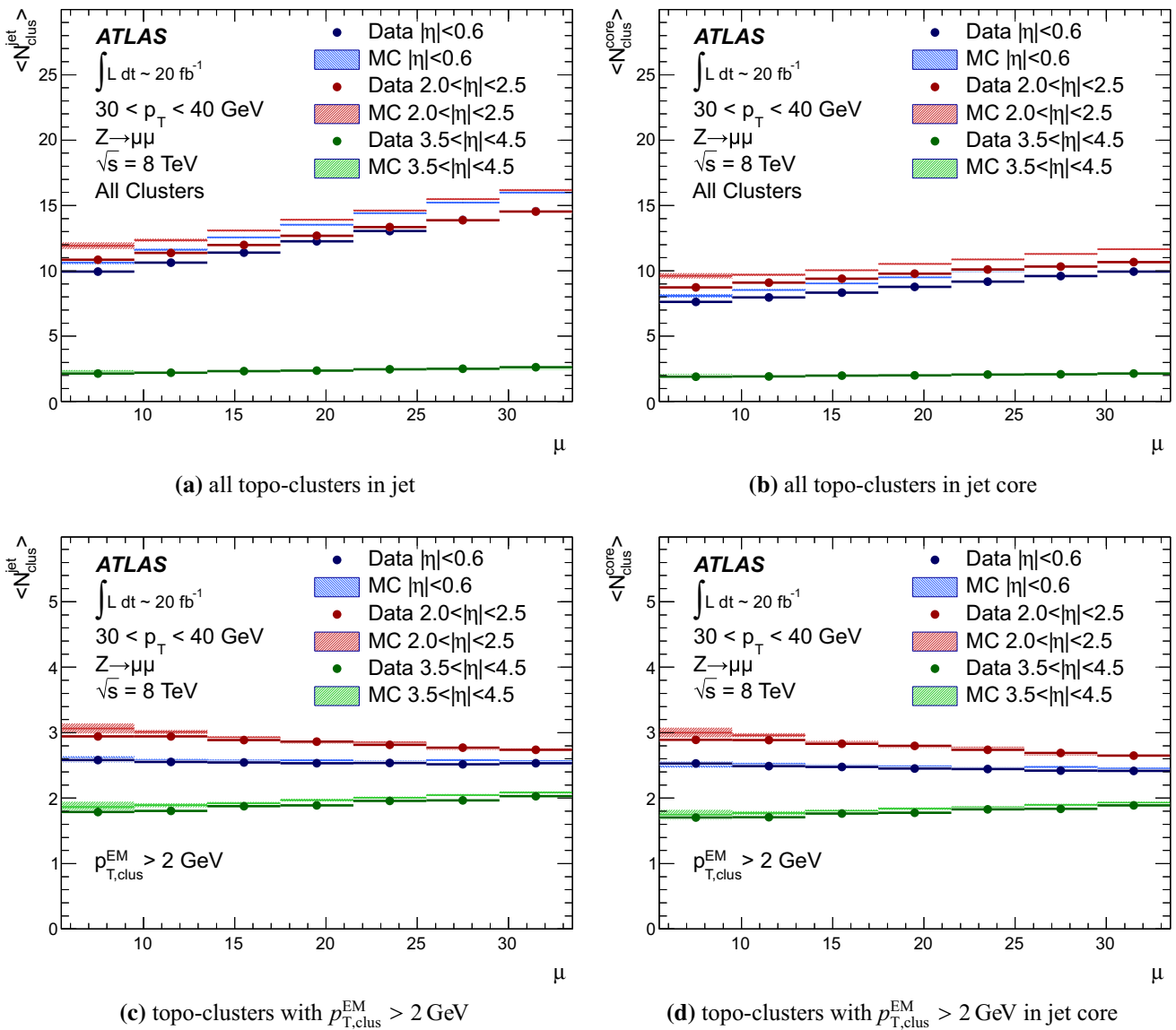
Fig. 33 The average number of topo-clusters \langle N_{clus}^{jet} \rangle in anti- k_r jets reconstructed with R = 0.4 within 30 \text{ GeV} < p_{T,jet}^{LCW+JES} < 40 \text{ GeV} as a function of \mu , in Z \rightarrow \mu\mu events in 2012 data and MC simulations (a) . The pile-up dependence of the average number of topo-clusters \langle N_{clus}^{core} \rangle in the core of the jet, defined by the distance to jet axis \Delta R < 0.3 ,
