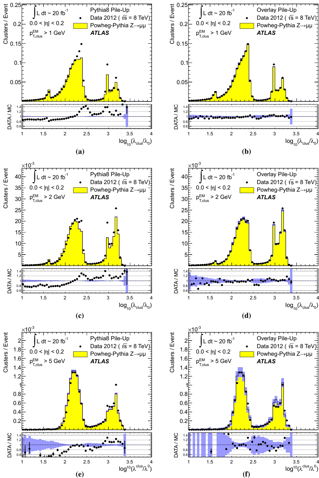
Fig. 29 The distribution of the topo-cluster depth location, measured in terms of \log_{10}(\lambda_{clus}/\lambda_0) , for selected topoclusters within |\eta_{clus}| < 0.2 and with a transverse momentum p_{T,clus}^{EM} , evaluated on the EM scale, larger than various thresholds. Results are shown for an inclusive Z \rightarrow \mu\mu event sample recorded in 2012. Data are compared to distributions from MC simulations including fully simulated pile-up for
