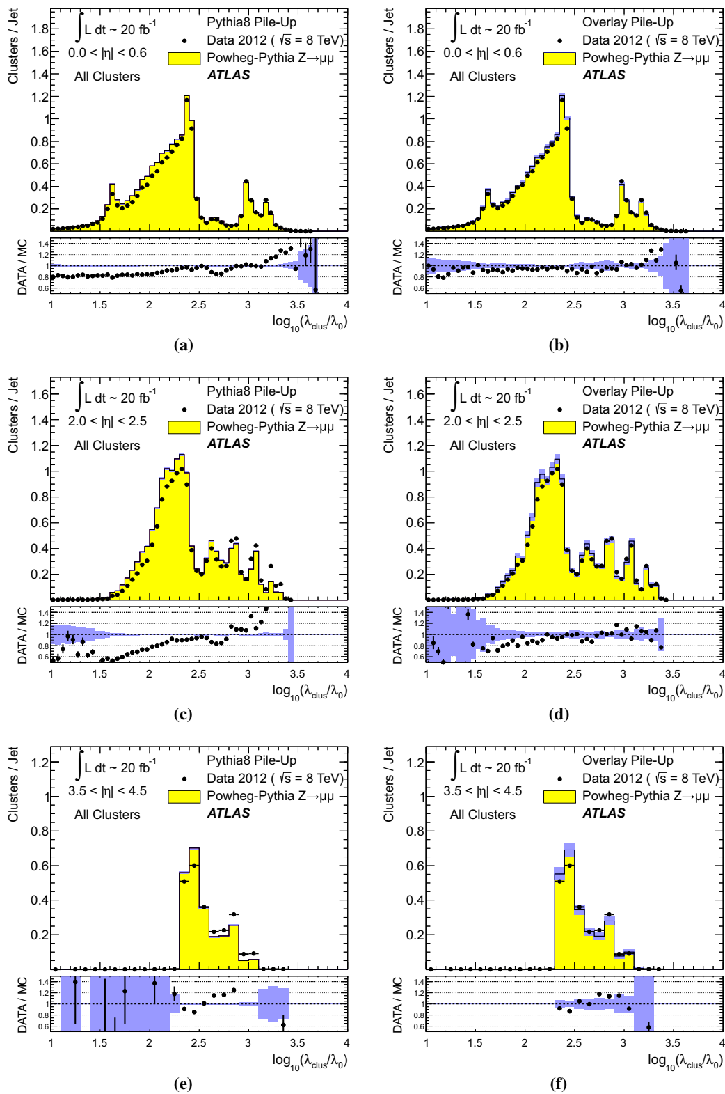
Fig. 34 The distribution of the depth location, measured in terms of \log_{10}(\lambda_{clus}/\lambda_0) with \lambda_0 = 1 mm, of all topo-clusters in jets reconstructed with the anti- k_r algorithm with R = 0.4 and with 30 \text{ GeV} < p_{T,jet}^{LCW+JES} < 40 \text{ GeV} in Z \rightarrow \mu\mu events in 2012 data and MC simulations with (a, c, e) fully simulated pile-up and with (b, d, f) overlaid pile-up from data. Distributions are shown for jets in the (a, b) central
