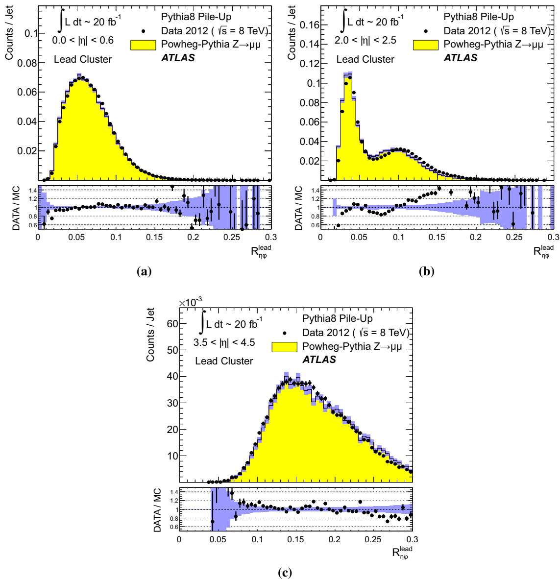
Fig. 43 The size R_{\eta\phi}^{lead} of the leading topo-cluster in (\eta, \phi) space, measured using Eq. (20), in anti- k_r jets reconstructed with R = 0.4 and with 30 \text{ GeV} < p_{T,jet}^{LCW+JES} < 40 \text{ GeV} in Z \rightarrow \mu\mu events in 2012 data and MC simulations with fully simulated pile-up. Distributions are shown for jets in the a central ( |\eta| < 0.6 ), the b end-cap ( 2.0 < |\eta| < 2.5 ), and
