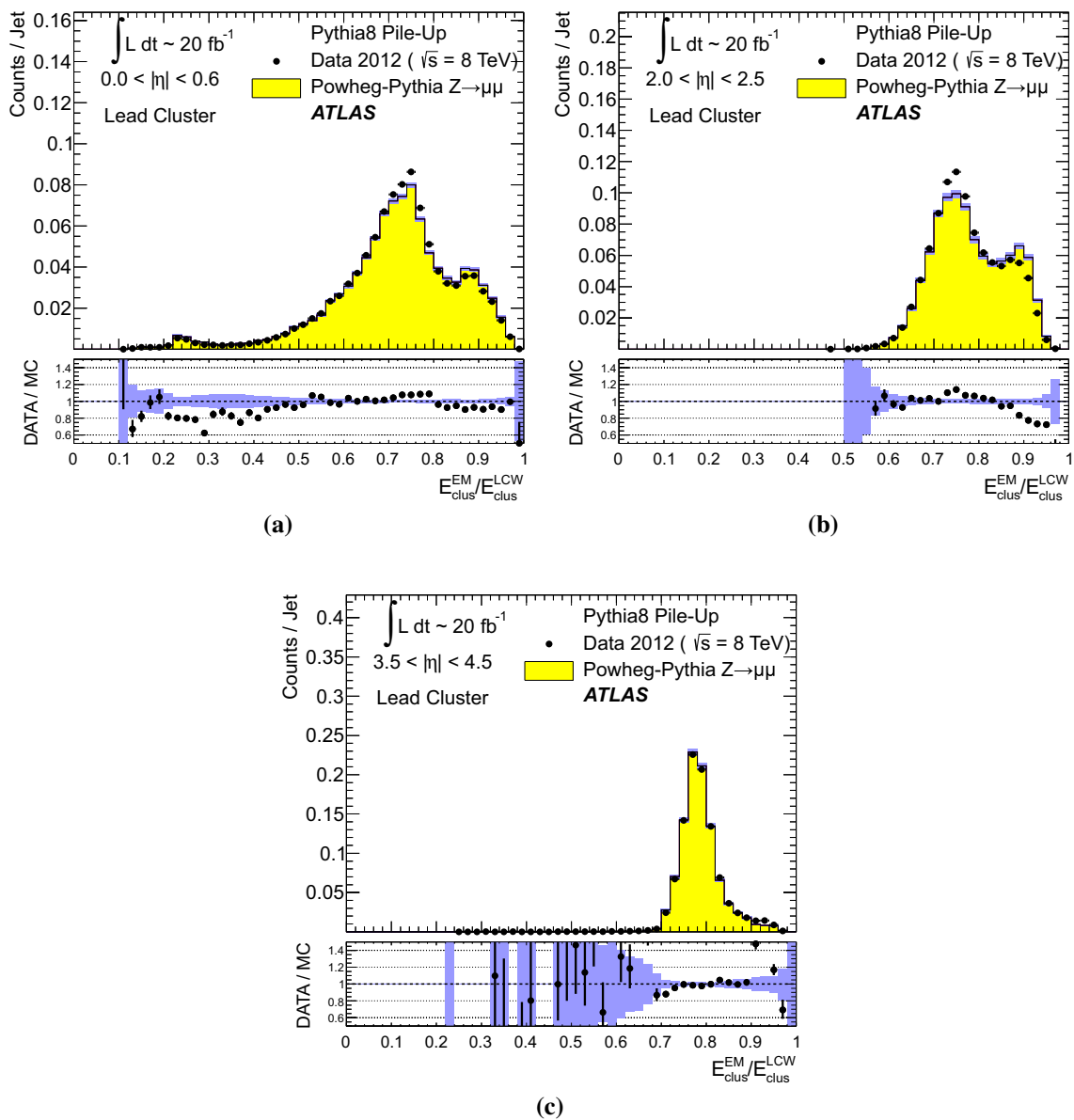
Fig. 38 The distribution of the ratio of the cluster signal reconstructed on EM scale E_{clus}^{EM} to the fully calibrated signal E_{clus}^{LCW} for the leading topo-cluster in fully calibrated jets reconstructed with the anti- k_r algorithm with R = 0.4 and 30 \text{ GeV} < p_{T,jet}^{LCW+JES} < 40 \text{ GeV} in regions of a the central ( |\eta_{jet}| < 0.6 ), b the end-cap ( 2.0 < |\eta_{jet}| < 2.5 ), and c the forward ( 3.5 < |\eta_{jet}| < 4.5 ) calorimeters in ATLAS. Data is compared
