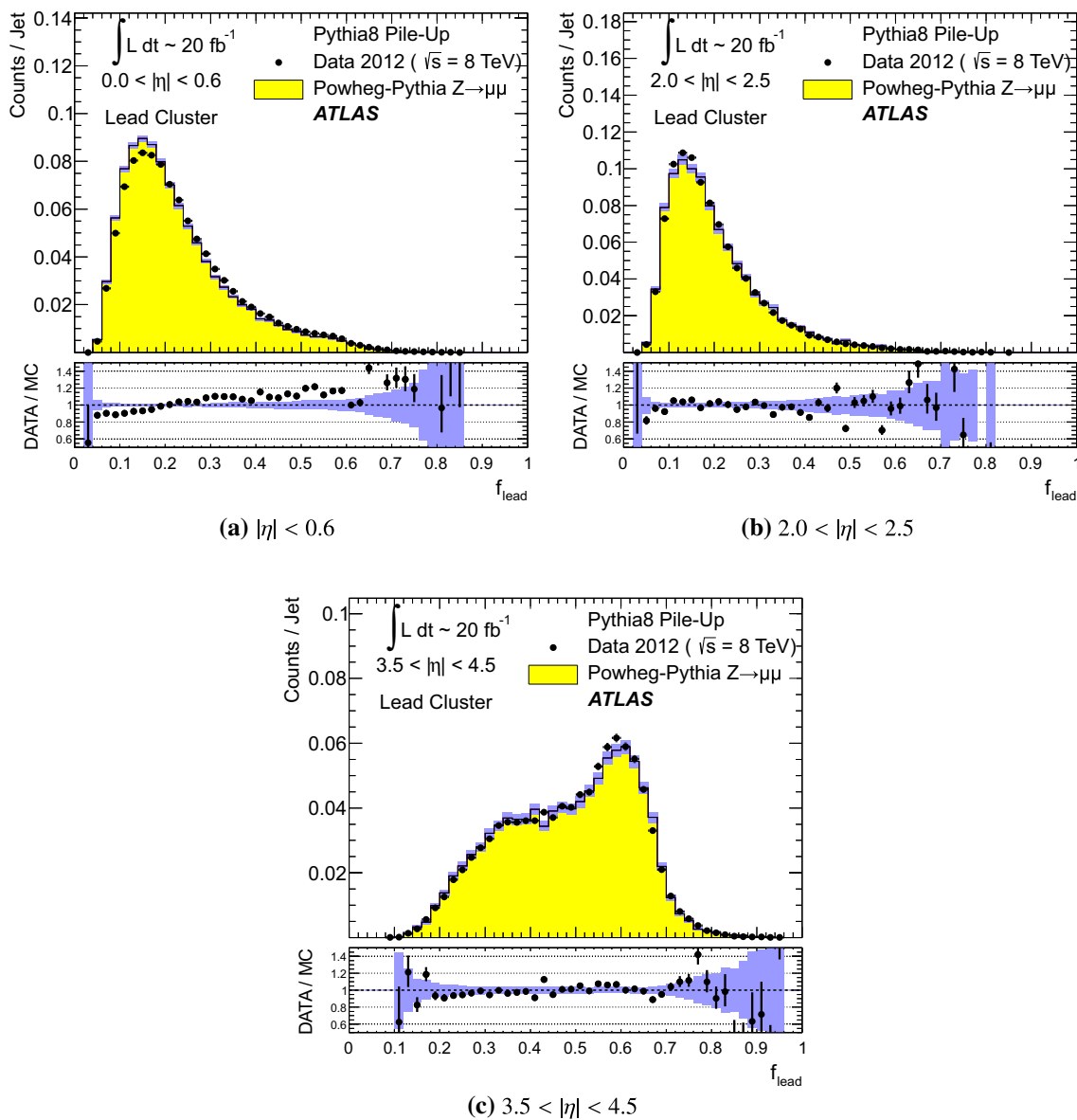
Fig. 39 The distribution of the signal fraction f_{lead} carried by the leading topo-cluster in jets, as defined in Eq. (45), in a the central, b the end-cap, and c the forward detector region. The jets are reconstructed using the anti- k_t algorithm with R = 0.4 and with 30 \text{ GeV} < p_{T,jet}^{LCW+JES} < 40 \text{ GeV} in Z \rightarrow \mu\mu events in 2012 data and
