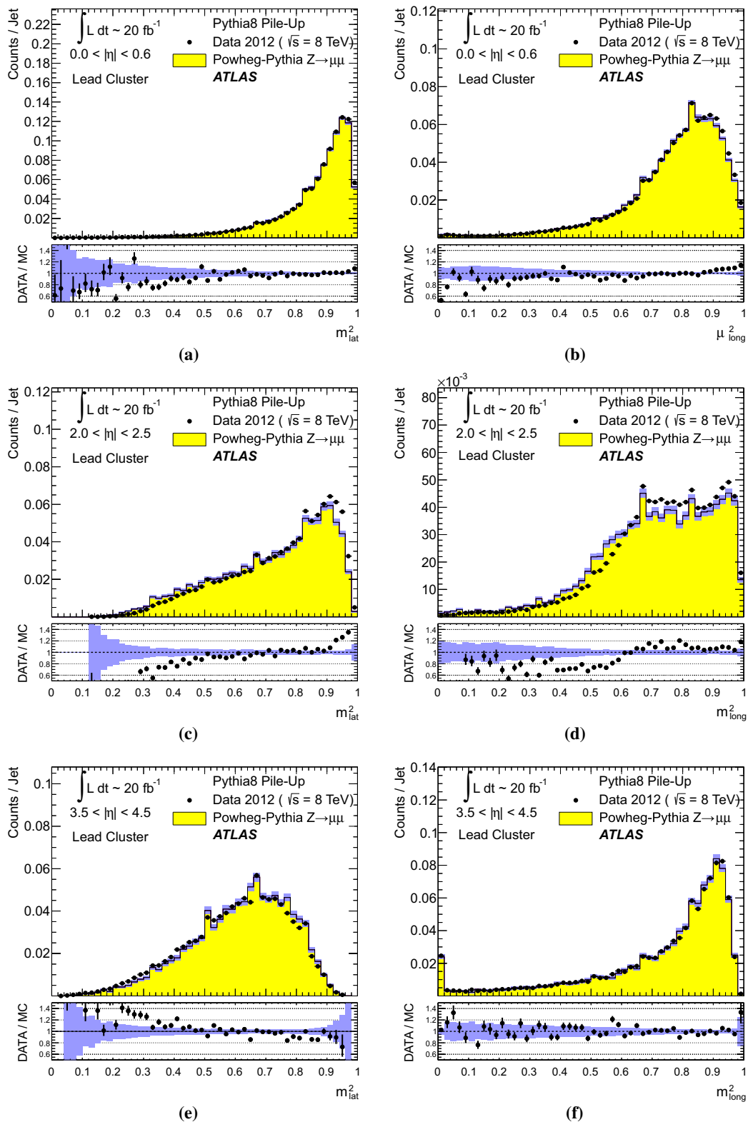
Fig. 41 The distribution of the normalised (a, c, e) lateral ( m_{lat}^2 ) and (b, d, f) longitudinal ( m_{long}^2 ) extension measures of the leading topo-cluster in fully calibrated anti- k_t jets with R = 0.4 and 30 \text{ GeV} < p_{T,jet}^{LCW+JES} < 40 \text{ GeV} in Z \rightarrow \mu\mu events in 2012 data and MC simulations with fully simulated pile-up, for jets in the (a, b) central ( |\eta| < 0.6 ), the (c, d) end-cap ( 2.0 < |\eta| < 2.5 ), and the (e, f)
