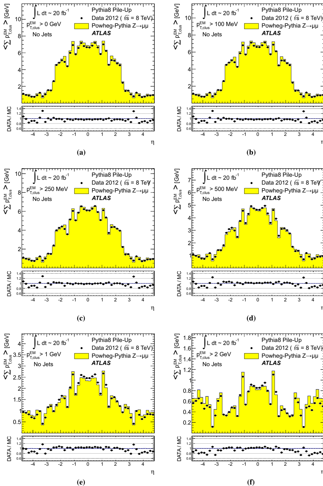
Fig. 23 The average \langle \sum p_{T,clus}^{EM} \rangle of clusters at the EM scale, calculated as function of \eta using Eq. (41), for clusters with a p_{T,clus}^{EM} > 0 , b p_{T,clus}^{EM} > 100 MeV, c p_{T,clus}^{EM} > 250 MeV, d p_{T,clus}^{EM} > 500 MeV, e p_{T,clus}^{EM} > 1 GeV, and f p_{T,clus}^{EM} > 2 GeV. Results are obtained from a
