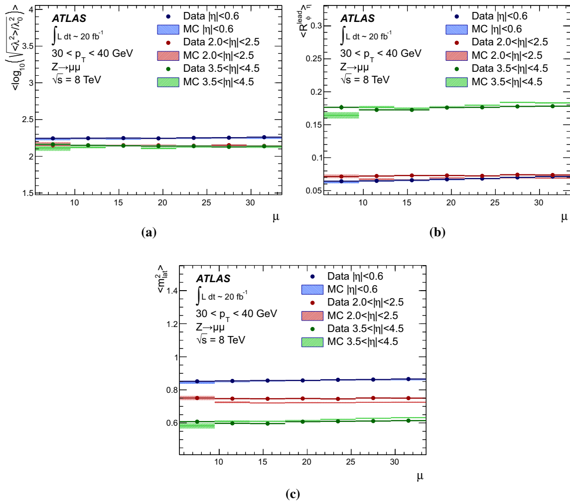
Fig. 44 The average pile-up dependence of various geometric observables reconstructed from the leading topo-cluster in anti- k_r jets reconstructed with R = 0.4 and 30 \text{ GeV} < p_{T,\text{jet}}^{\text{LCW+JES}} < 40 \text{ GeV} in Z \rightarrow \mu\mu events in 2012 data and MC simulations with fully simulated pile-up. The average cluster length, represented by \log_{10} \left( \left( \frac{\lambda^2}{\lambda_0^2} \right)^{1/2} \right) with the reference scale \lambda_0 = 1 \text{ mm} , is shown as a function of \mu in a , for three detector regions. The average size \langle R_{\eta\phi}^{\text{lead}} \rangle of the lead-
