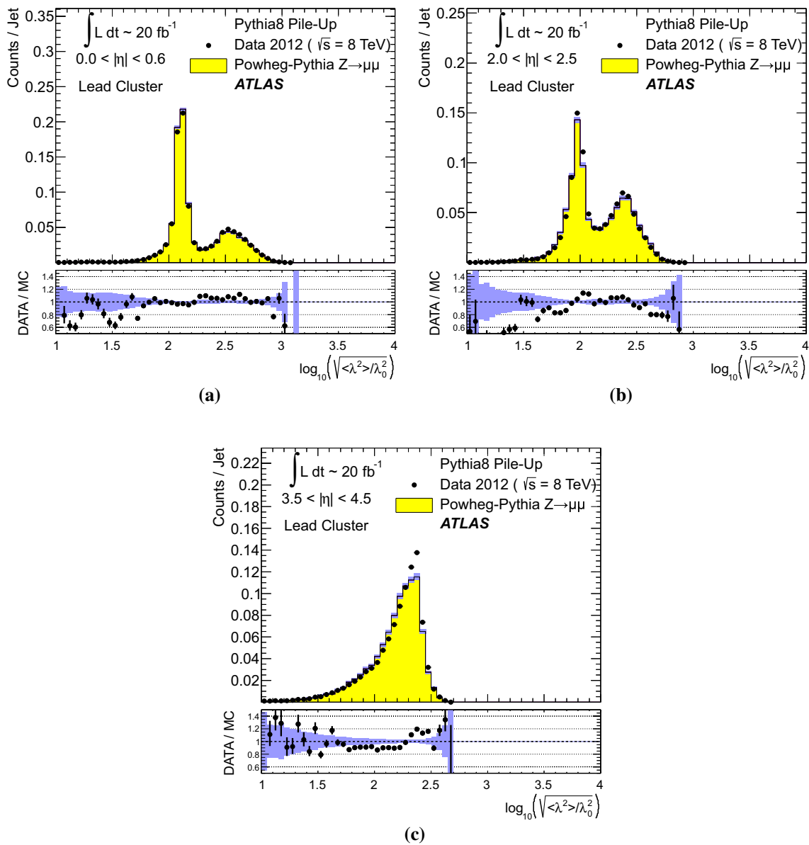
Fig. 42 The length of the leading topo-cluster, measured in terms of the longitudinal spread (second moment) ( \lambda^2 ) of the cell coordinates along the principal cluster axis by \sqrt{\langle \lambda^2 \rangle / \lambda_0^2} , in anti- k_t jets reconstructed with R = 0.4 and 30 \text{ GeV} < p_{T,\text{jet}}^{\text{LCW+JES}} < 40 \text{ GeV} in Z \rightarrow \mu\mu events in 2012 data and MC simulations with fully simulated pile-up. Distributions are shown for jets in the a central ( |\eta| < 0.6 ), the b end-cap
