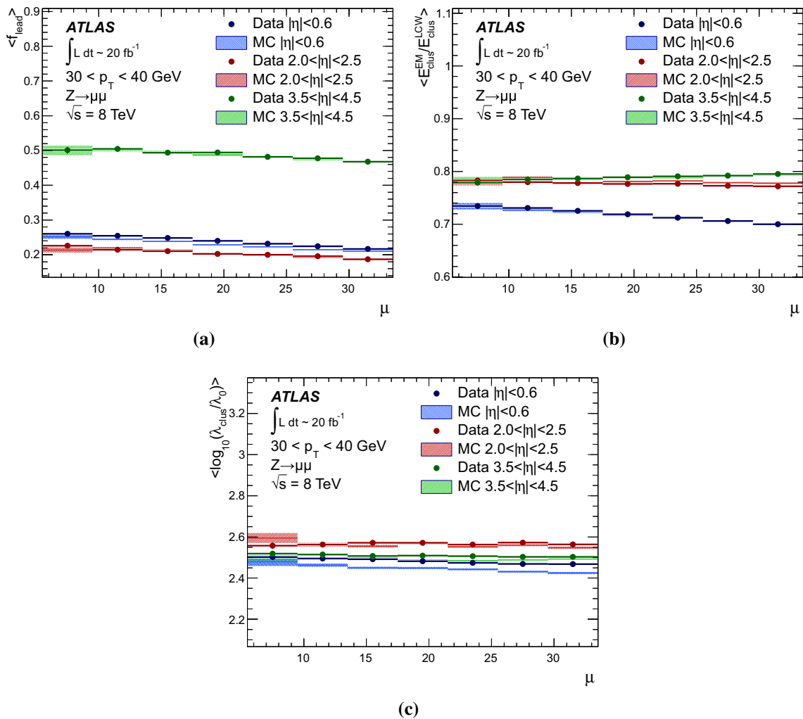
Fig. 40 The pile-up dependence of a f_{\text{lead}} defined in Eq. (45), b E_{\text{clus}}^{\text{EM}}/E_{\text{clus}}^{\text{LCW}} , and c the depth location \lambda_{\text{clus}} of the leading topo-cluster in fully calibrated anti- k_r jets reconstructed with R = 0.4 and with 30 \text{ GeV} < p_{\text{T,jet}}^{\text{LCW+JES}} < 40 \text{ GeV} in Z \rightarrow \mu\mu events in 2012 data
