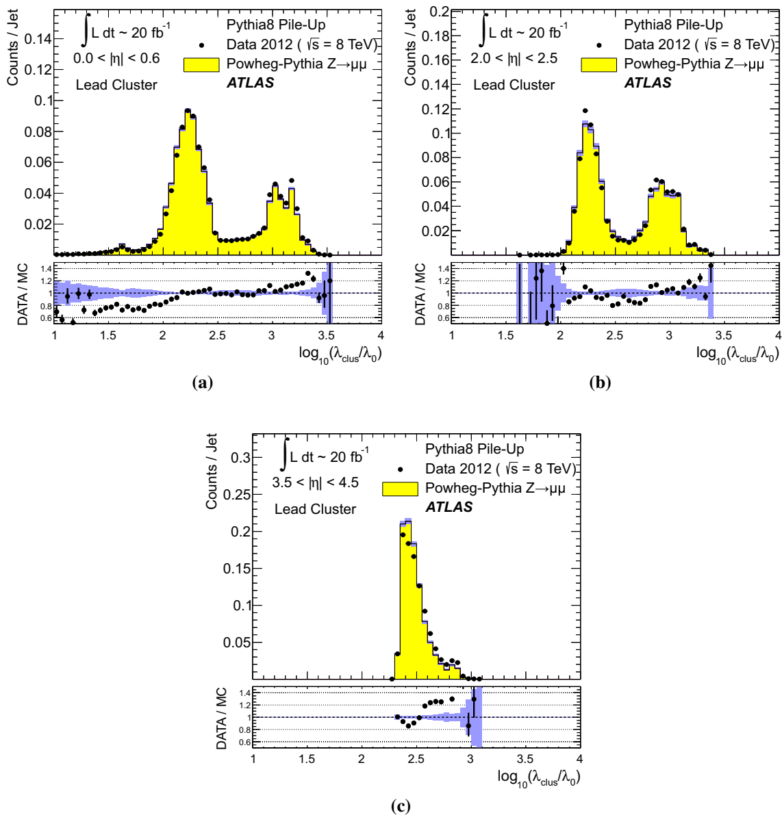
Fig. 36 The distribution of the leading topo-cluster depth location measure \log_{10}(\lambda_{\text{clus}}/\lambda_0) in fully calibrated jets reconstructed with the anti- k_r algorithm with R = 0.4 and 30\text{ GeV} < p_{T,\text{jet}}^{\text{LCW+JES}} < 40\text{ GeV} in regions of a the central ( |\eta_{\text{jet}}| < 0.6 ), b the end-cap ( 2.0 < |\eta_{\text{jet}}| < 2.5 ), and the c forward ( 3.5 < |\eta_{\text{jet}}| < 4.5 ) calorimeters in ATLAS. Data is compared to MC simulations with
