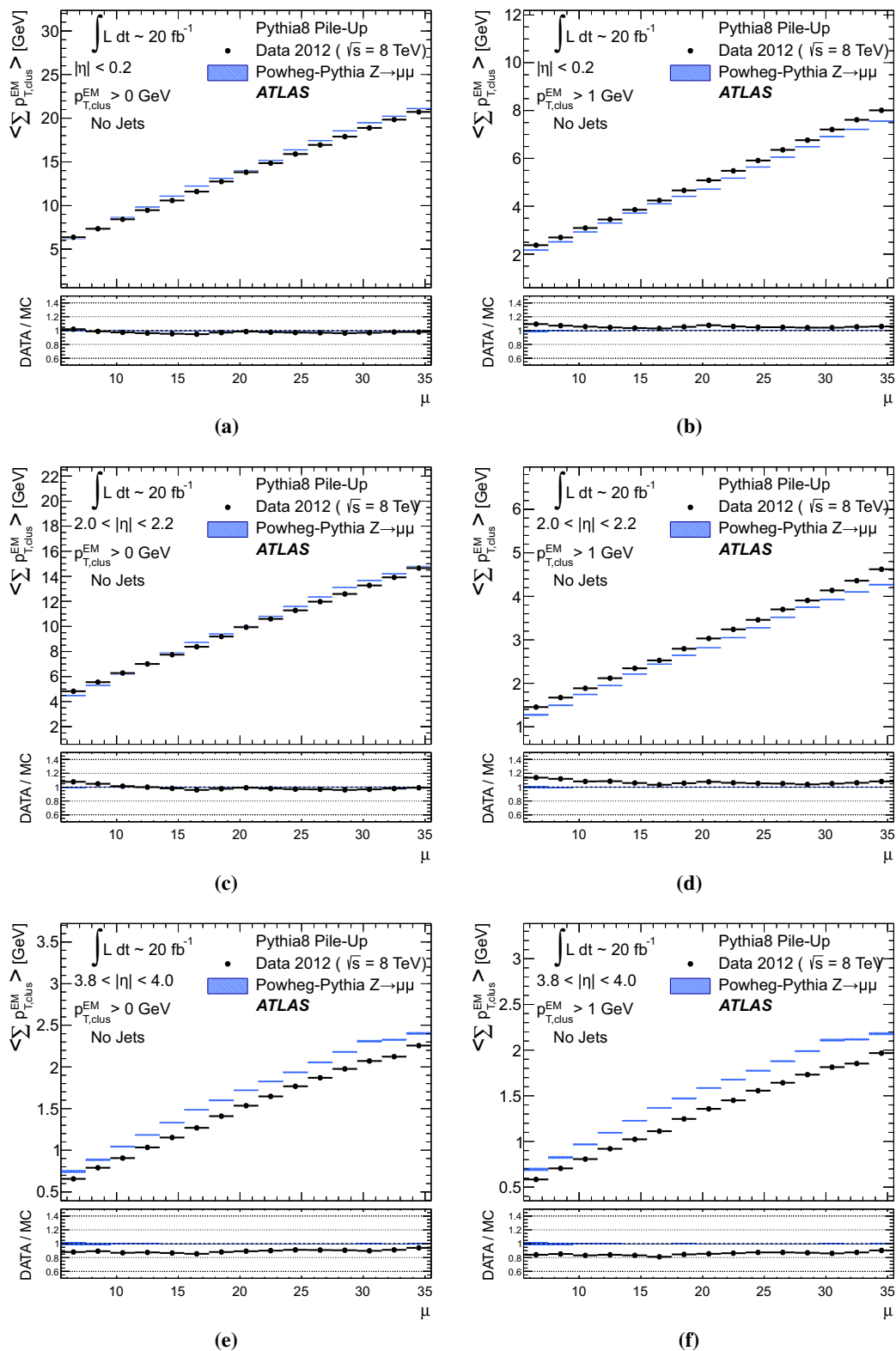
Fig. 24 The average transverse momentum flow \langle \sum p_{T,clus}^{EM} \rangle evaluated as function of the pile-up activity measured by the number of proton-proton interactions per bunch crossing \mu , in several calorimeter regions. In a , c , and e , \langle \sum p_{T,clus}^{EM} \rangle(\mu) is shown in the central ( |\eta| < 0.2 ), end-cap ( 2.0 < |\eta| < 2.2 ), and the forward ( 3.8 < |\eta| < 4.0 ) region, respectively, using topo-clusters with p_{T,clus}^{EM} > 0 . The corresponding results
