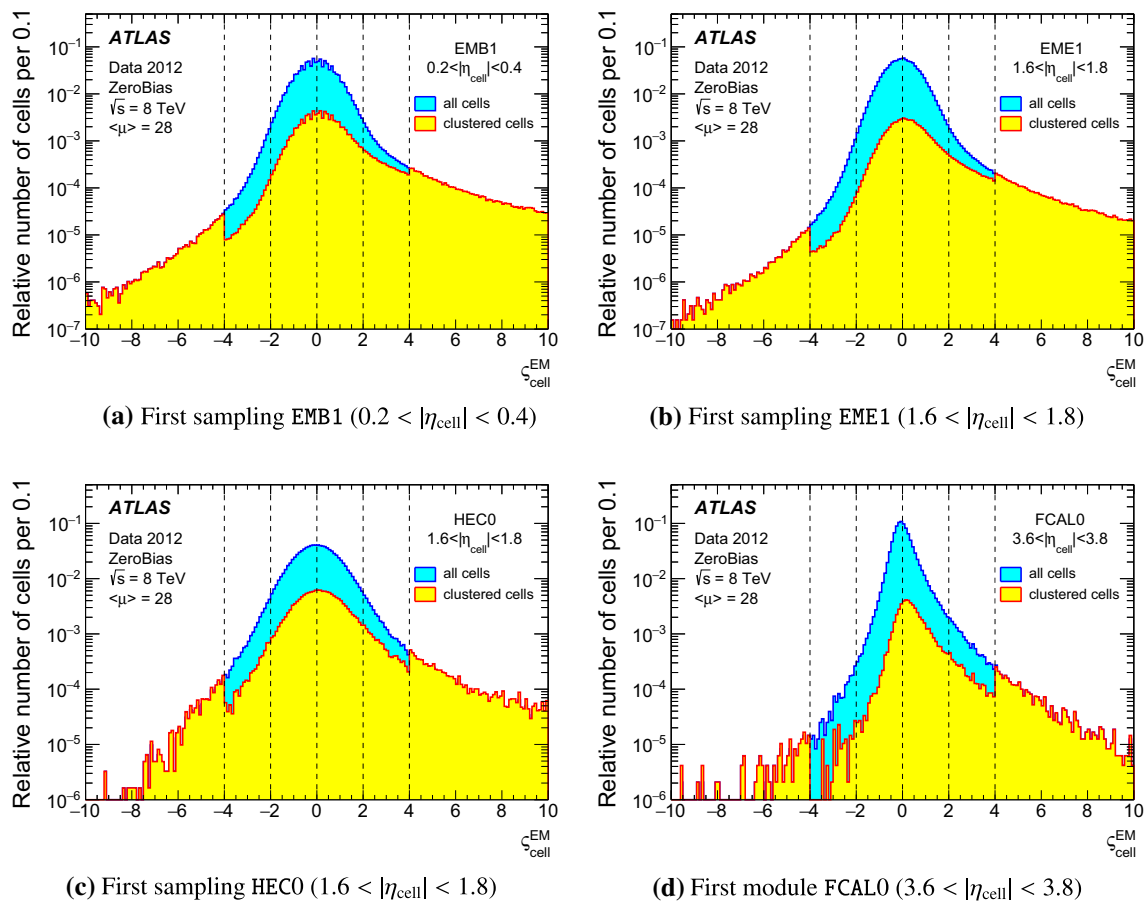
Fig. 5 Signal significance ( c_{\text{cell}}^{\text{EM}} ) distributions for all cells (blue/cyan) and for cells after the noise suppression in the topological cell clustering is applied (red/yellow), in selected sampling layers of the LAr calorimeters: a the first sampling of the central electromagnetic LAr calorimeter (EMB), b the first sampling of the electromagnetic LAr
