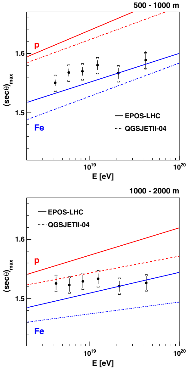
FIG. 9. Comparison between (\sec\theta)_{\max} , for both data and Monte Carlo predictions in the 500–1000 m interval (top) and in the 1000–2000 m interval (bottom) using both hadronic models EPOS-LHC (solid lines) and QGSJETII-04 (dashed lines), for both primaries, proton (red) and iron (blue).
