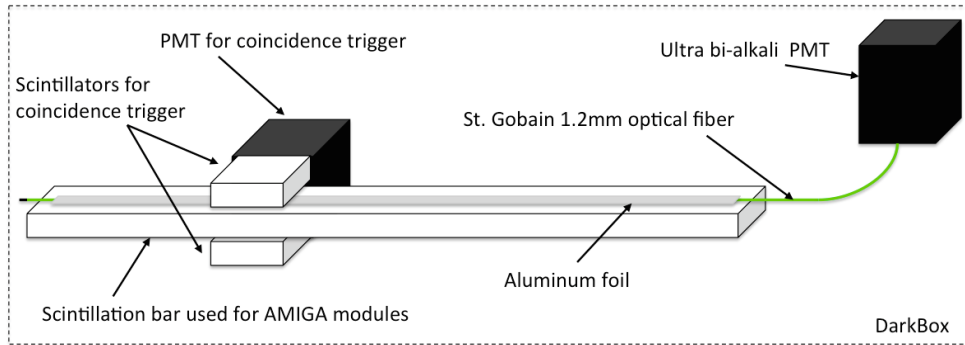
Figure 6. Setup to measure the number of SPEs produced per muon. Two 4\text{ cm} \times 4\text{ cm} \times 1\text{ cm} scintillator bars and a regular multi-anode PMT were used to generate a coincidence trigger. A 5 m Saint-Gobain fiber was glued within the groove of a 4 m scintillation bar and curved-up at one end to optically connect it to a PMT.
