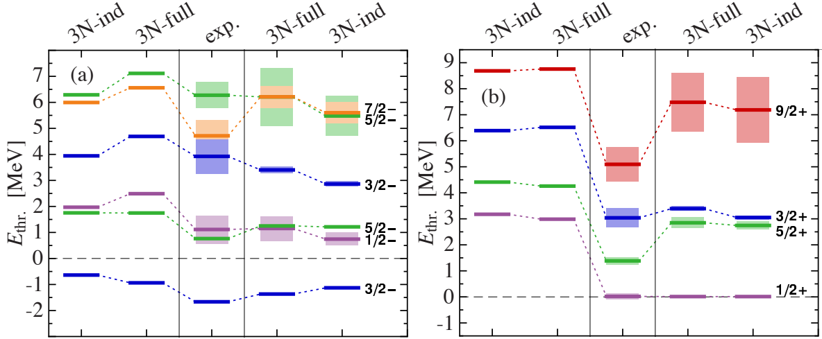
Figure 20. Negative (a) and positive (b) parity spectrum of {}^9\text{Be} relative to the n\text{-}{}^8\text{Be} threshold at N_{\text{max}} = 12 and 11 , respectively. Shown are NCSM (first two columns) and NCSMC (last two columns) results compared to experiment [150]. First and last columns contain the energies for the NN+3N-ind and the second and fourth column for the NN+3N-full Hamiltonian, respectively. Shaded areas denote the width of the energy levels. Remaining parameters are \hbar\Omega = 20 MeV and \Lambda = 2.0 fm ^{-1} . Figure taken from [144].
