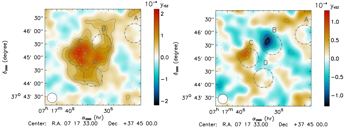
Fig. 5. Map of the thermal SZ effect, y_{tSZ} (left), and the kinetic SZ effect, y_{kSZ} (right). Gray contours are multiples of 1\sigma , starting at \pm 2\sigma . The map effective resolution, 22 arcsec, is shown as a white circle on the bottom left corner. Subcluster regions are represented in gray. The positions of the identified point sources (see Sect. 3), from which mis-subtraction residuals remain a potential local contaminant to the signal, are represented in light gray.
