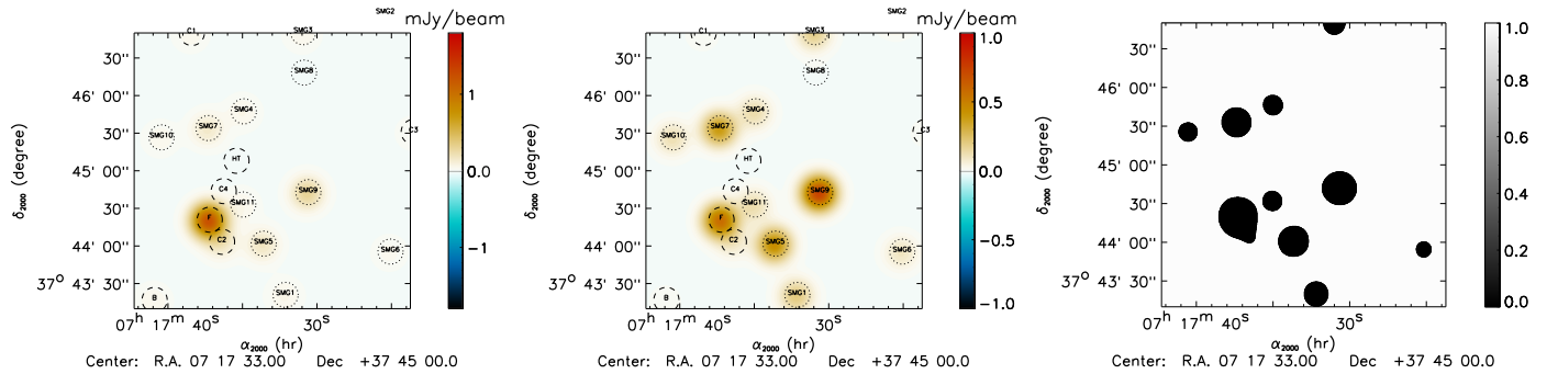
Fig. 2. Point source model at 150 GHz ( left ) and 260 GHz ( middle ), and point source mask constructed from the 150 and 260 GHz point source models ( right ). The color scale of the models is the same as in Fig. 1. We also provide the labels of each source on the figure, in dashed circles for radio sources and dotted circles for submillimeter sources. The point sources subtracted maps can be seen in Fig. 7.
