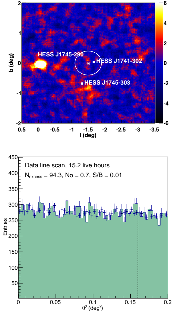
FIG. 1. Significance map presented in Galactic coordinates ( top ) and emission angle square ( \theta^2 ) distribution ( bottom ) in the considered ROI. The ROI is expressed in the map with a white circle centred on the 130 GeV excess ( -1.5^\circ, 0^\circ ) marked with a white cross. The known source HESS J1745-290 is detected, even at large angular offset. The dashed vertical line in the bottom shows the \theta cut of 0.4^\circ .
