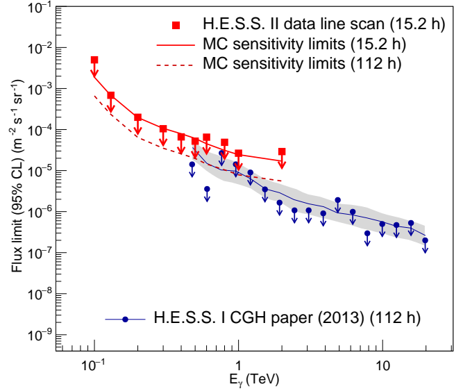
FIG. 2. Flux limits at 95% CL for a line scan between 100 GeV and 2 TeV. The results obtained from 15.2 h of data are represented by points in red. The red dashed line represents the limits expected for 112 h of observation time, calculated as the median limits from 500 simulated data sets. The red solid line is given for 15.2 h MC simulations. Former limits from H.E.S.S. I [3] obtained in the Central Galactic Halo (CGH) region are represented as blue data points (the grey band displaying the level of systematic uncertainties).
