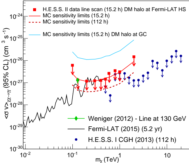
FIG. 3. \langle\sigma v\rangle limits at 95% CL (red points) for the line scan between 100 GeV and 2 TeV, derived from 15.2 h of data and using an Einasto DM profile with \Phi_{astro} value calculated with CLUMPY package [25] ( \rho_s = 20 kpc, r_s = 0.17 ). The MC estimations are presented with the same conventions as in Figure 2. Former limits from H.E.S.S. I [3] obtained in the CGH region and Fermi-LAT [10] are represented by blue and black data points, respectively. The \langle\sigma v\rangle value corresponding to the 130 GeV line feature reported as R16 in [7] is shown in green. The limits extracted with assumption of the DM halo position at the GC are shown with a continuous blue line (see in the text). It should be noted that the comparison of the limits on the hotspot obtained in this work can not be directly done with the H.E.S.S. I results as DM halo was centred on the Galactic Centre position in the sky. In case of Fermi-LAT , the red curve can still be compared to the Fermi-LAT limits as the latter would only be marginally modified (at the level of 1%) by the displacement of the DM halo, given the very large size of the ROI ( 16^\circ of radius) in use.
