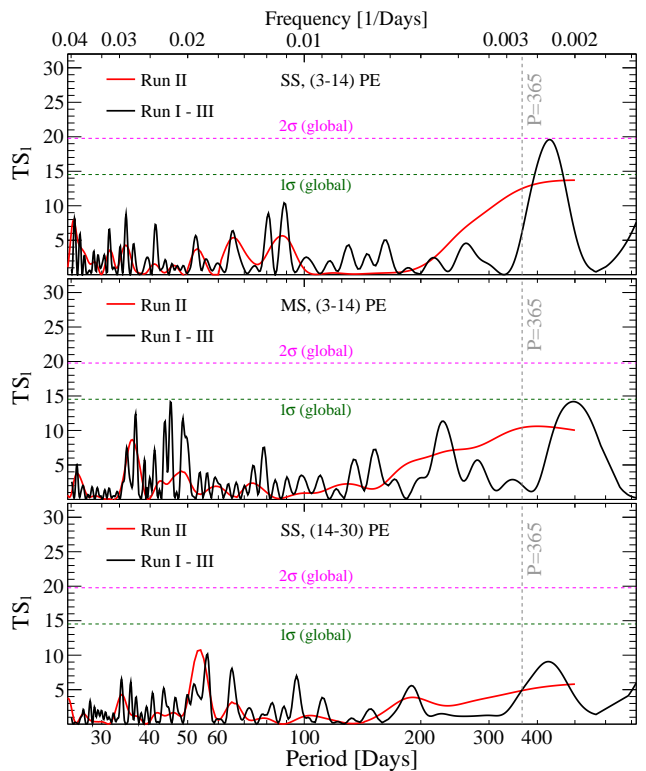
FIG. 4. Test statistics as a function of modulation period for single scatters in the low-E region (top), multiple scatters in the low-E region (middle) and single scatters in the high-E region (bottom). The phase is unconstrained. The previous Run II-only result [12] is overlaid for comparison.
