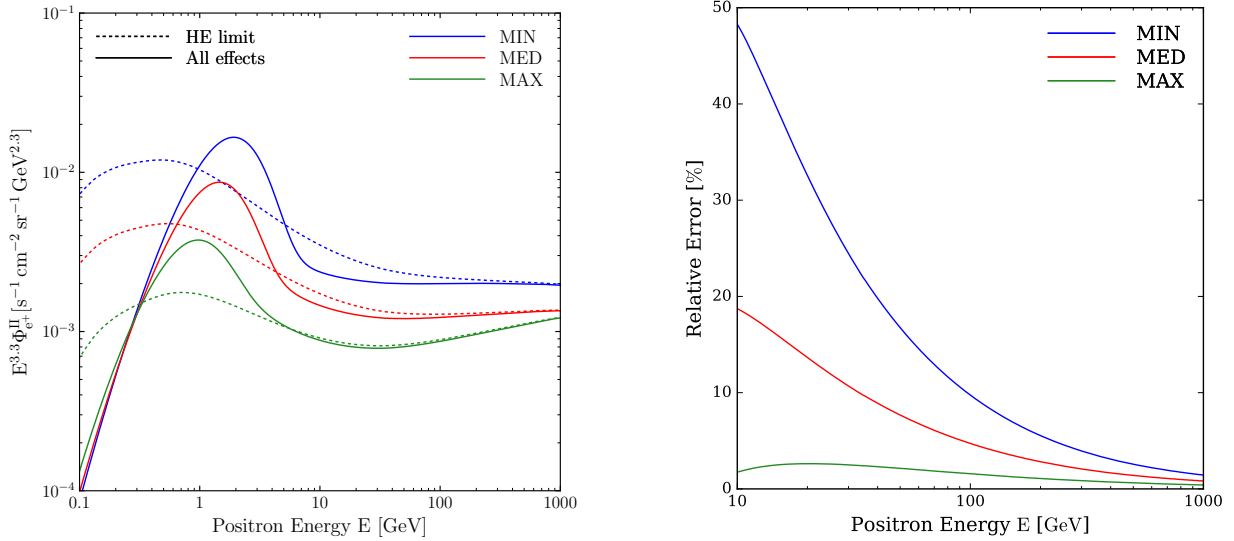
Fig. 6. Left panel: interstellar flux (multiplied by E^{3.3} ) of secondary positrons computed with all propagation effects ( \Phi_{\text{HE}}^{\text{II}} , solid lines) and with the high-energy approximation ( \Phi_{\text{HE}}^{\text{II}} , dotted lines) for the MIN (blue), MED (red), and MAX (green) models. Right panel: relative error (\Phi_{\text{HE}}^{\text{II}} - \Phi^{\text{II}})/\Phi^{\text{II}} above 10 GeV of the high-energy approximation for secondary positrons compared to the exact result.
