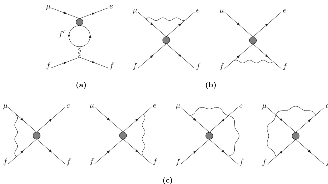
Figure 1. One-loop Feynman diagrams for the mixing of the four-fermion lepton-quark and lepton-tau operators.
