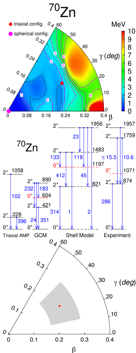
FIG. 9. (Color online) (top) Potential Energy Surface from constrained Hartree-Fock minimization in the shell-model basis for ^{70}\text{Zn} . (middle) Level scheme and B(E2\downarrow) values (in MeV and e^2\text{fm}^4 , respectively) for different theoretical models described in the text and from the present experiment (except for the 2_3^+ state observed in another work and whose B(E2) value is unknown). (bottom) 1\sigma contours in the \beta - \gamma sextant for the ground-state of ^{70}\text{Zn} . The red dot represents the effective \beta and \gamma value.
