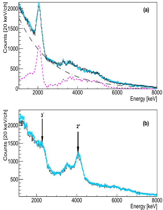
FIG. 5. (Color online) (a): Doppler-corrected and background-subtracted \gamma -ray spectrum conditioned by the detection of scattered ^{68}\text{Ni} in the DSSSD (black histogram). The number of counts in the 2_1^+ state at 2.034 MeV was extracted by using the simulated response function of the detection system (dashed magenta line). The curve in blue circles corresponds to the global fit, which includes an exponential decay (long-dashed gray line), the excitations of the 3^- and 2_1^+ states in ^{208}\text{Pb} , and high-energy contributions discussed in Sect. III B 3. (b): Same as (a), but for the non Doppler-corrected spectrum. The decays of the 3^- and 2_1^+ states in ^{208}\text{Pb} are visible at 2.614 and 4.085 MeV (with single-escape), respectively, for which our measured B(E3) and B(E2) values agree with the ones of the literature.
