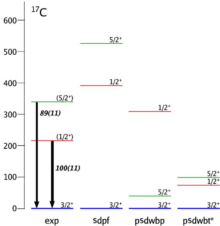
Figure 2.11: Low lying level scheme of ^{17}\text{C} [30]. Different theoretical calculations for WBP and modified WBT interactions are shown.
