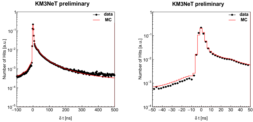
Figure 4.4: The difference between the true and expected time of arrival for hits assuming a muon hypothesis, averaged over all events in the sample, compared against the Monte Carlo expectation for atmospheric muons. The distribution has been normalised so that the sum of each bin over the full range (left) is equal to one.
