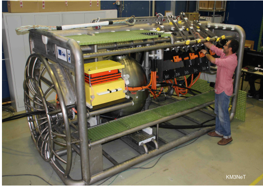
Figure 2.15: The first KM3NeT/ORCA junction box, photographed at CPPM before deployment.
