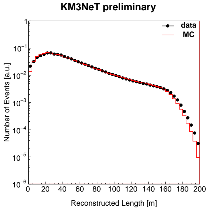
Figure 4.5: The reconstructed track length distributuion for data in selected runs, compared against the Monte Carlo expectation for atmospheric muons.
