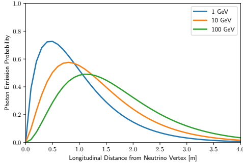
Figure 2.5: The parameterised longitudinal photon emission profiles of EM cascades in water for various energies.
