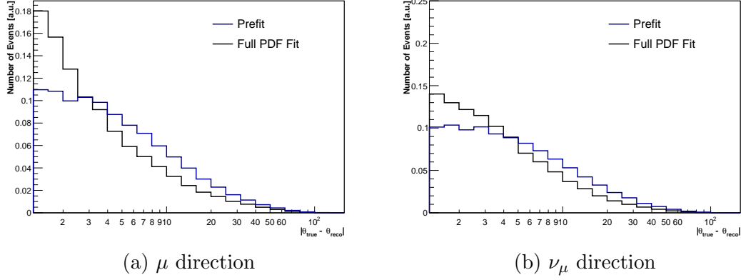
Figure 3.9: The zenith uncertainty in degrees for \nu_\mu -CC interactions, weighted with the unoscillated Honda flux, reconstructed with the full ORCA detector, where the reconstructed track begins inside the detector volume. It is shown with respect to both the neutrino direction and outgoing muon direction for the prefit and full PDF fit stages of the reconstruction chain.
