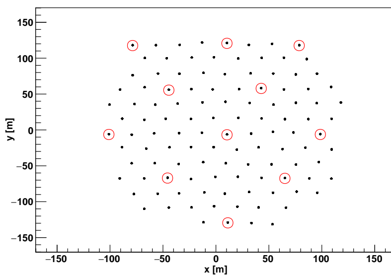
Figure 4.3: The ORCA detector footprint with selected DUs highlighted with a red circle.
