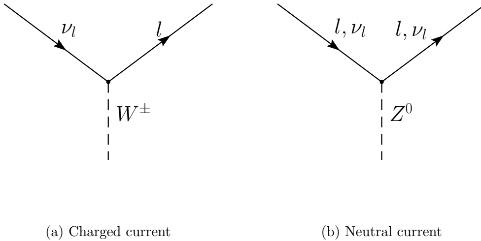
Figure 1.1: Two neutrino interaction weak interaction vertices, where l denotes any of the three charged leptons.
