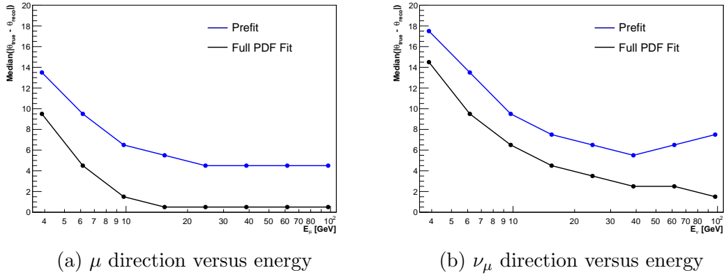
Figure 3.10: The median zenith uncertainty in degrees for \nu_\mu -CC interactions, weighted with the unoscillated Honda Flux, reconstructed with the full ORCA detector, where the reconstructed track begins inside the detector volume. It is shown with respect to the both the neutrino direction and outgoing muon for direction for the prefit and full PDF fit stages of the reconstruction chain. Above muon energies of 10 GeV, \nu_\mu direction uncertainty is dominated by the kinematic angle between the muon and the neutrino.
